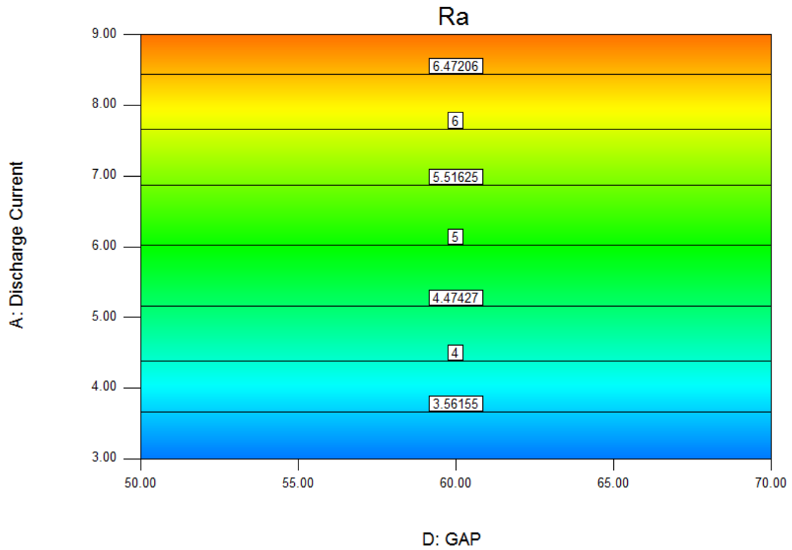
Fig- 8. Contour plot: Discharge current vs. Gap.
