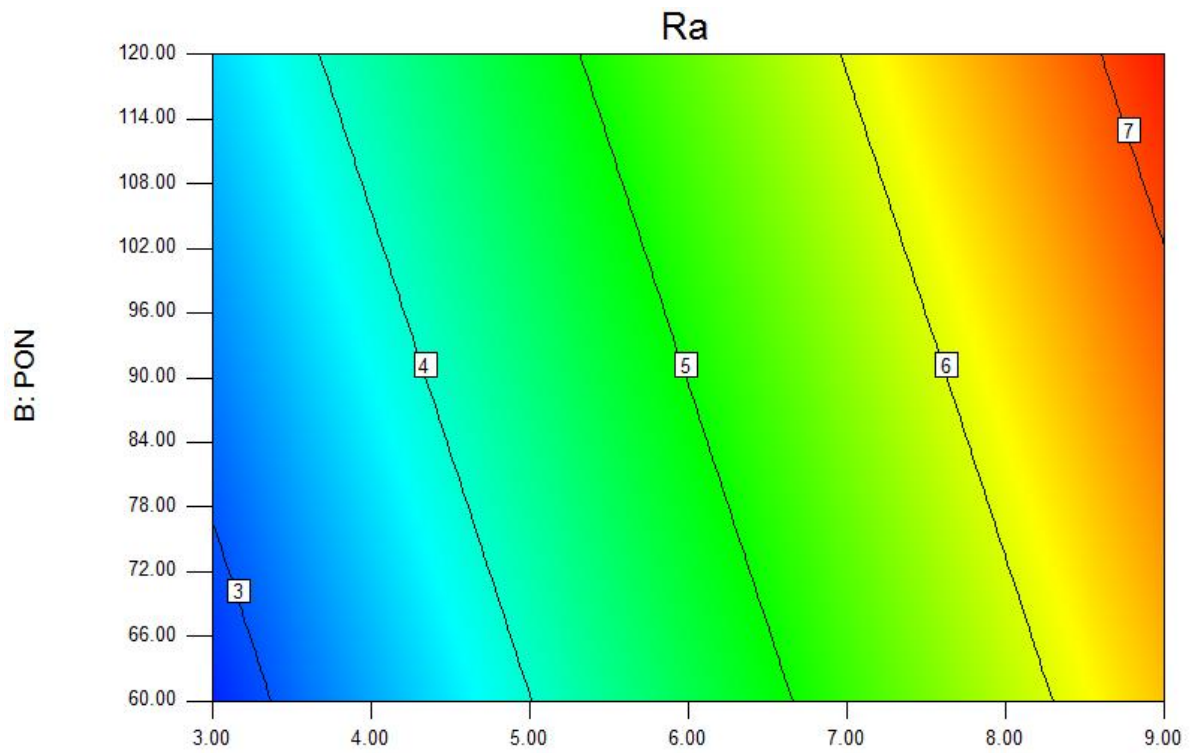
A: Discharge Current Fig- 6. Contour plot: Discharge current vs. PON.
