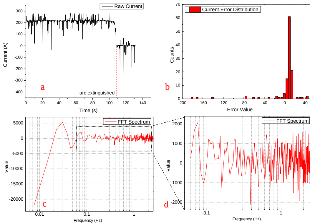
Figure 16a. Raw current signal for a single layer; 16b. error histogram for current data after arc extinguished 16c. fast Fourier Transformed Current Spectrum;
