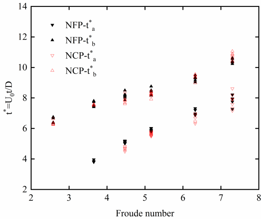
Fig. 9 Non-dimensional pinch-off time as a function of the Froude number for NFP and NCP.
