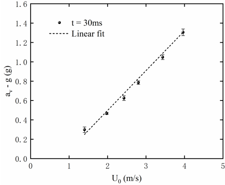
Fig. 8 Axial impact acceleration, normalized by g as a function of the initial velocity U_0 for NFP at the moment of 30 ms.
