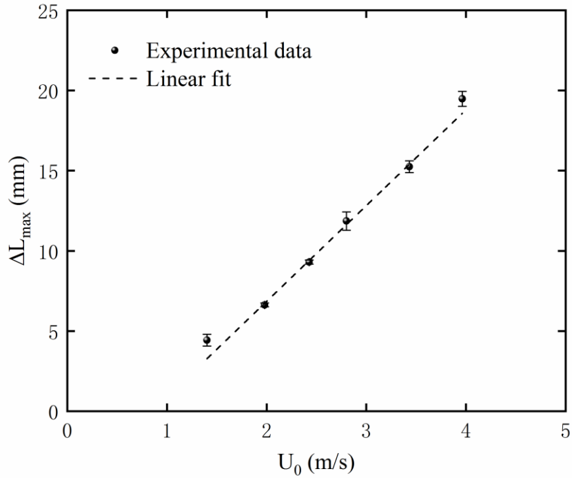
Fig. 11 Maximum compression \Delta L_{\max} as a function of the initial velocity U_0 for NCP during the initial stage of impact.
