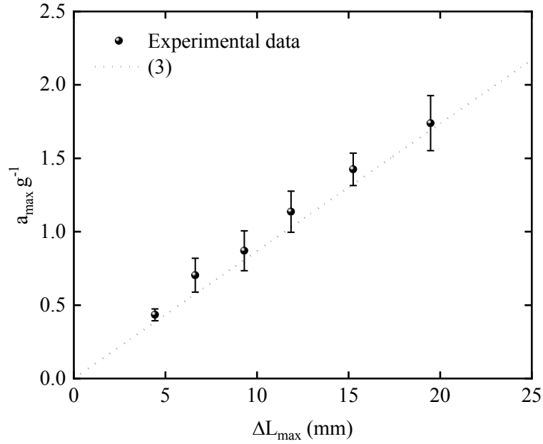
Fig. 14 Maximum impact acceleration a_{\max} as a function of the maximum deformation \Delta L_{\max} for NCP during the initial stage of impact.
