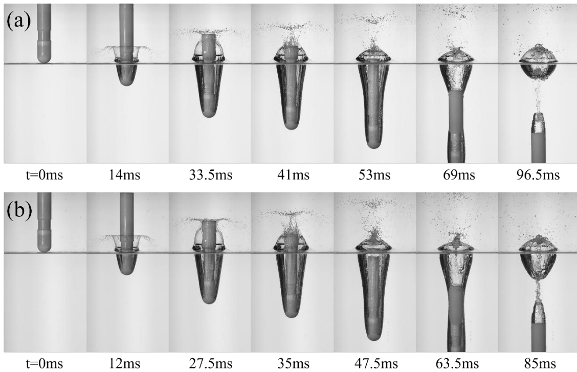
Fig. 5 Image sequence of water entry for NFP. (a) U_0 = 3.43 m/s, the surface closure appears first on the side of the projectile at the time of 33.5ms and then again on the tail at the time of 53ms. (b) U_0 = 3.96 m/s, the surface closure appears first on the side of the projectile at the time of 27.5ms and then again on the tail at the time of 47.5ms.
