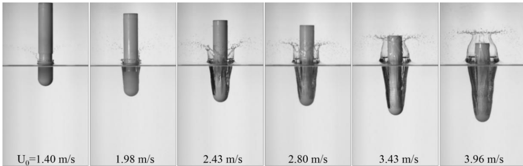
Fig. 12 Instantaneous water entry events of NCP with different initial velocities at the time of 32.5 ms
