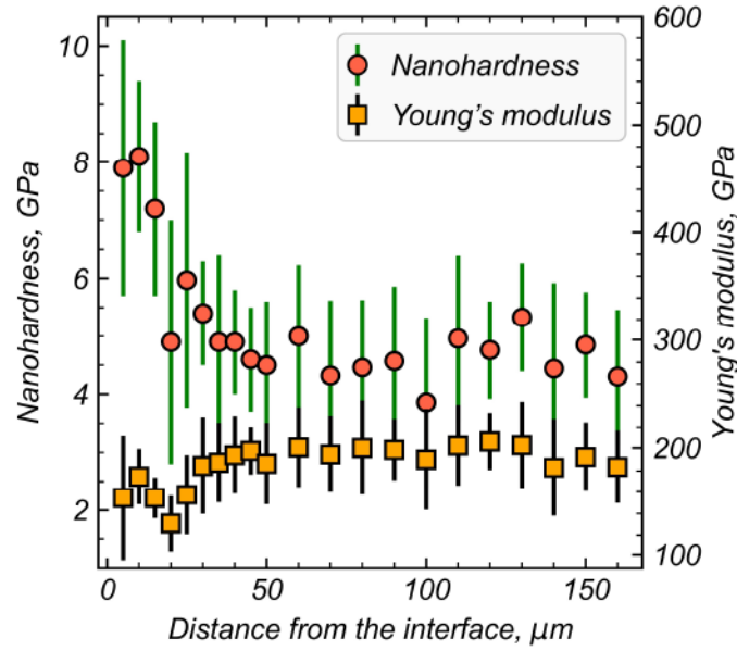
Figure 12: Nanohardness and Young's modulus of the sample after 500 friction cycles.
