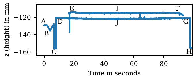
Figure 4. In-process RRI time series of layer five recorded during deposition of the sixth layer. The z -axis values show the reference plate (A), the v-shaped trough (B, added by CNC motion system rather than a real feature of the target), the build platform (C) beneath the build plate, the build plate (D) continuing through the start of the wall (E), since the plot shows the point cloud at all positions across the wall, see figure 5), the end of the wall (F) and the end of the build plate (G), and the build platform (H). The signal levels indicated by I and J represent measurement of the wall and build plate at different galvo scan angles (figure 5 occurs across points I and J. Isolated points between the wall top and the build plate correspond to intermittent measurement of the sides of the wall).
