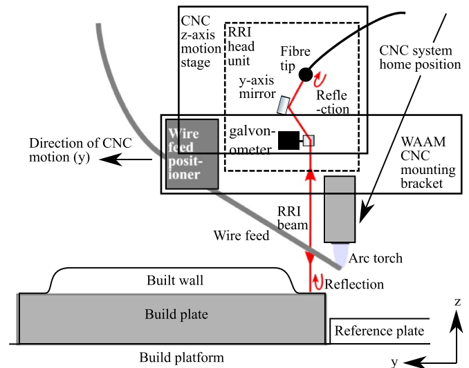
Figure 3. Diagram (not to scale) showing the build geometry and WAAM CNC mounting bracket (attached to the CNC z -axis motion stage, itself suspended from above) holding wire feed positioner, arc torch and RRI head unit. The CNC motion system home position, far above and to the right of the build plate, is shown. An RRI time series recorded during the deposition of the sixth layer (and therefore measuring the fifth layer ahead of the arc torch and WAAM deposition) is shown in figure 4. The diagram is shown from the side, i.e. from the perspective of the camera shown in figure 2.
