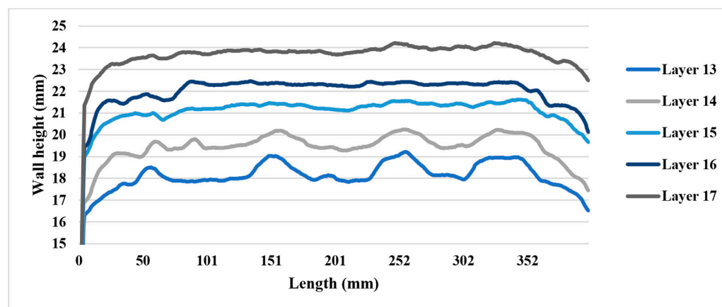
Figure 14. Average wall height variation of layers 13 to 17.
