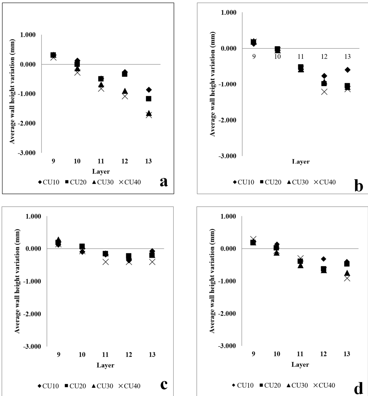
Figure 7. Variation in wall height with increasing wire feed speed with different process parameters. (a) Wall #5: Current: 200 Amp; TS: 6 mm/s. Base layer parameter: WFS: 90 mm/s. CUs parameters: WFS 60 mm/s. (b) Wall #6: Current: 200 Amp; TS: 6 mm/s. Base layer parameter: WFS: 90 mm/s. CUs parameters: WFS 75 mm/s. (c) Wall #7: Current: 250 Amp; TS: 6 mm/s. Base layer parameter: WFS: 90 mm/s. CUs parameters: WFS 60 mm/s. (d) Wall #8: Current: 250 Amp; TS: 6 mm/s. Base layer parameter: WFS: 90 mm/s. CUs parameters: WFS 75 mm/s. .
