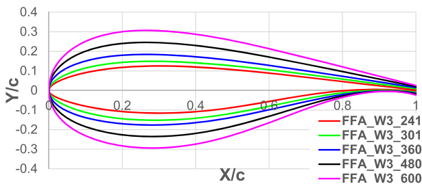
Fig. 1. FFA-W3 series aerofoils used for the 2D studies.
