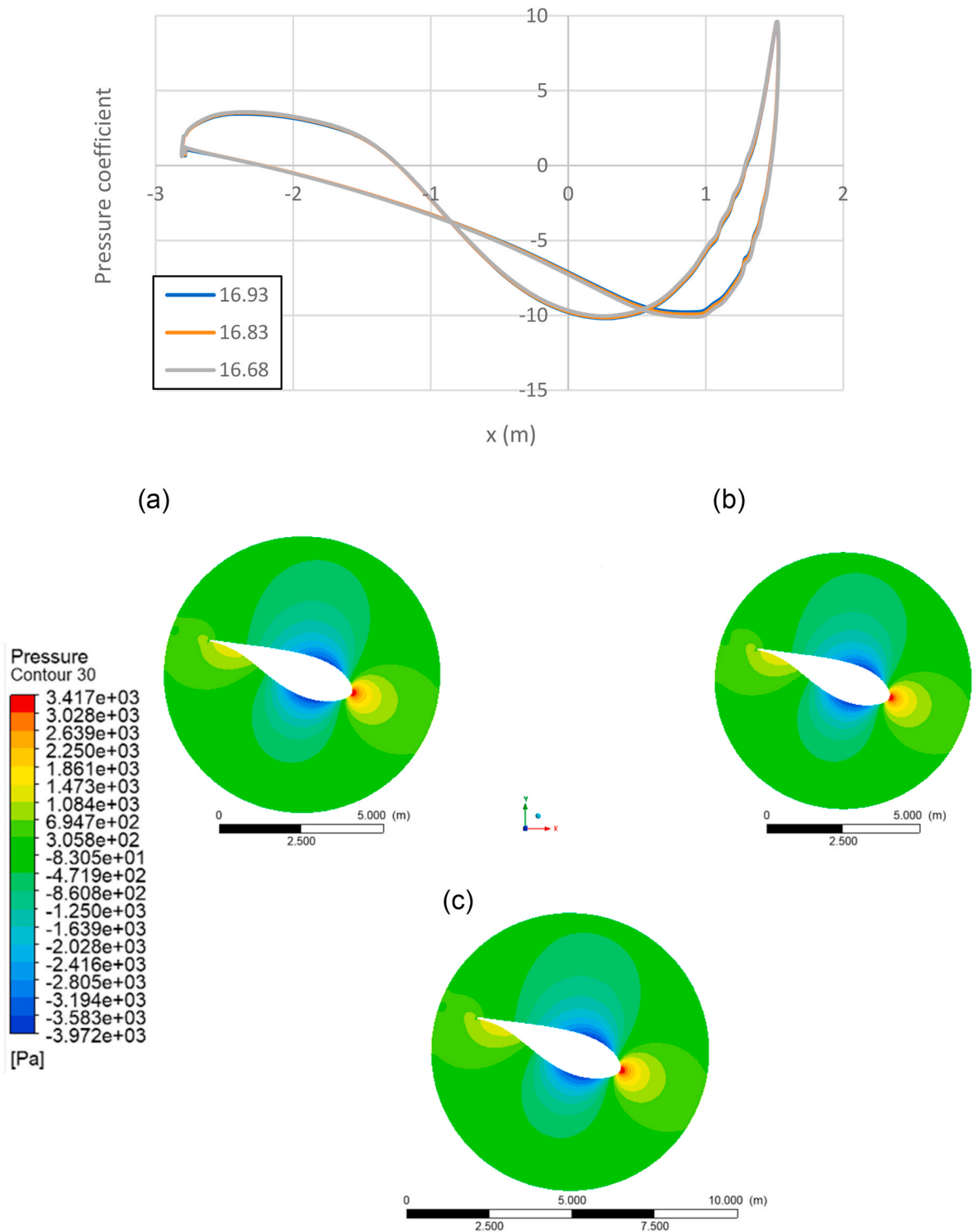
Fig. 12. At velocity 25 m/s pressure coefficient C_p and pressure contour plots for 25 m/s at different pitch angle (a) 16.93° (b) 16.83° (c) 16.68° at 60 % blade span.
