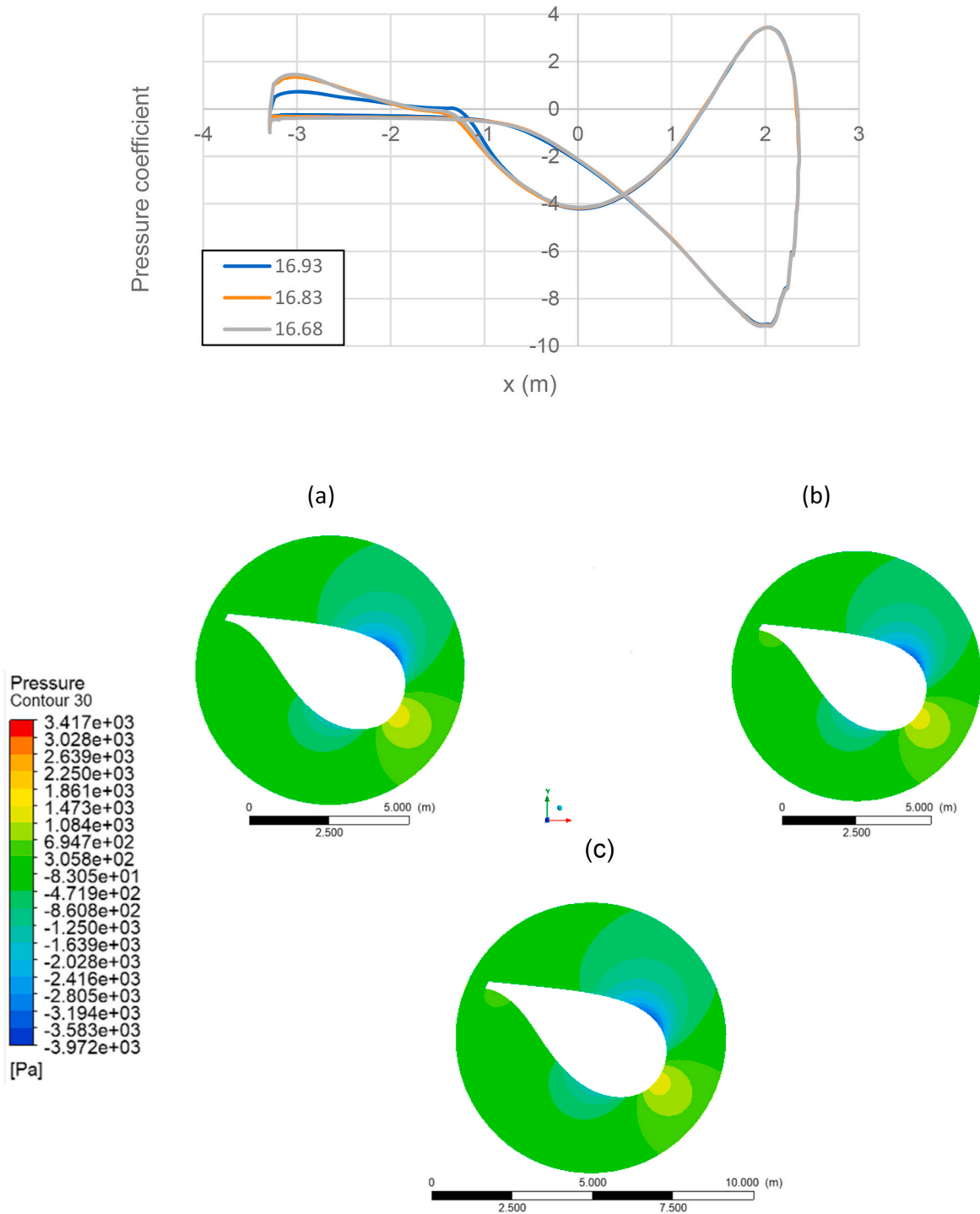
Fig. 11. At velocity 25 m/s pressure coefficient C_p and pressure contour plots for 25 m/s at different pitch angle (a) 16.93° (b) 16.83° (c) 16.68° at 30 % blade span.
