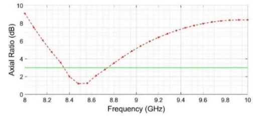
Figure 3 Simulated Axial Ratio of the proposed antenna.
