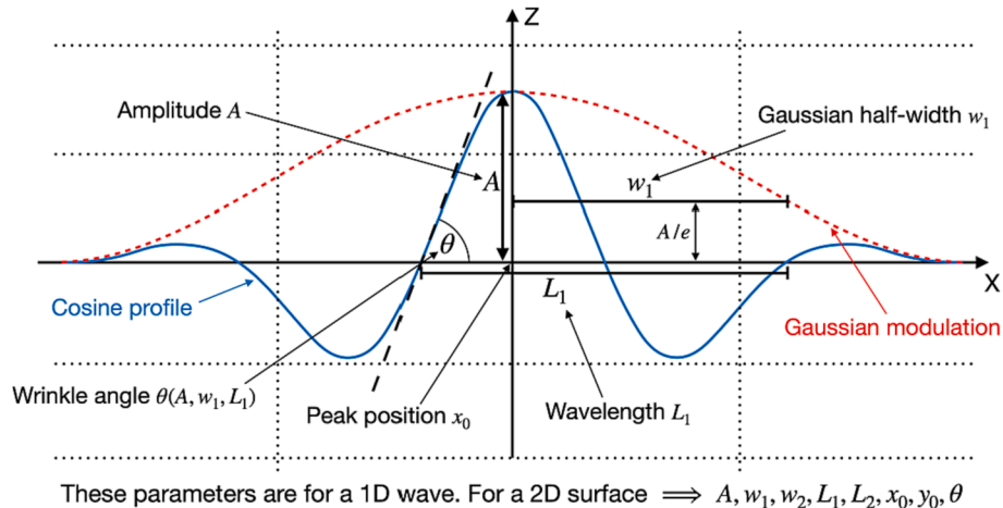
Fig. 2. Definition of wrinkle parameters for the proposed mathematical model of the waviness defect. The definition of such surface is expressed in Eq. (1), which outlines a relationship between the following eight wrinkle parameters (highlighted in Fig. 2, for the x-z projection only):
