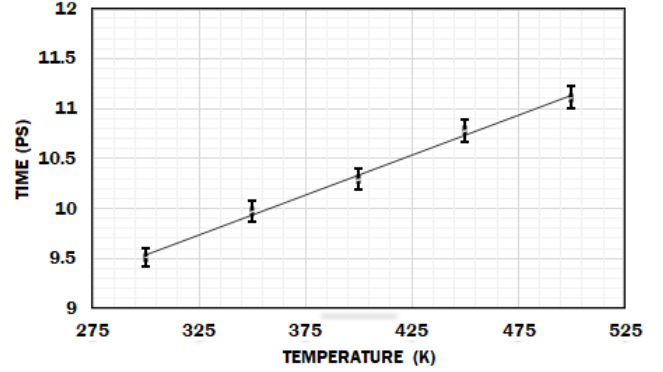
Fig 2. The effect of temperature on the period of transit of a Gunn domain in the planar structure.
