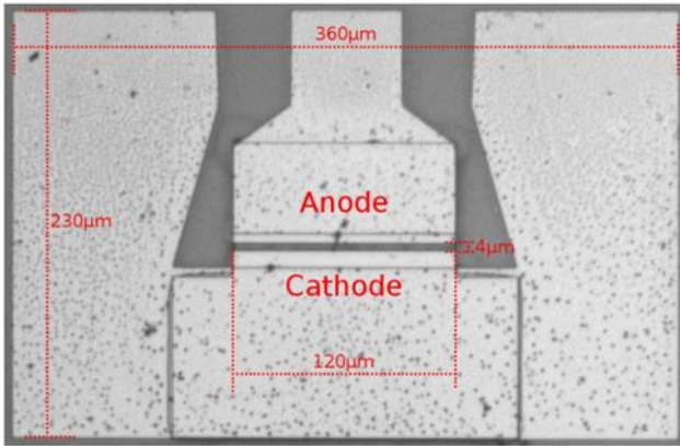
Fig. 1. Planar Gunn Diode with a 4x120 \mu\text{m} channel [10].
