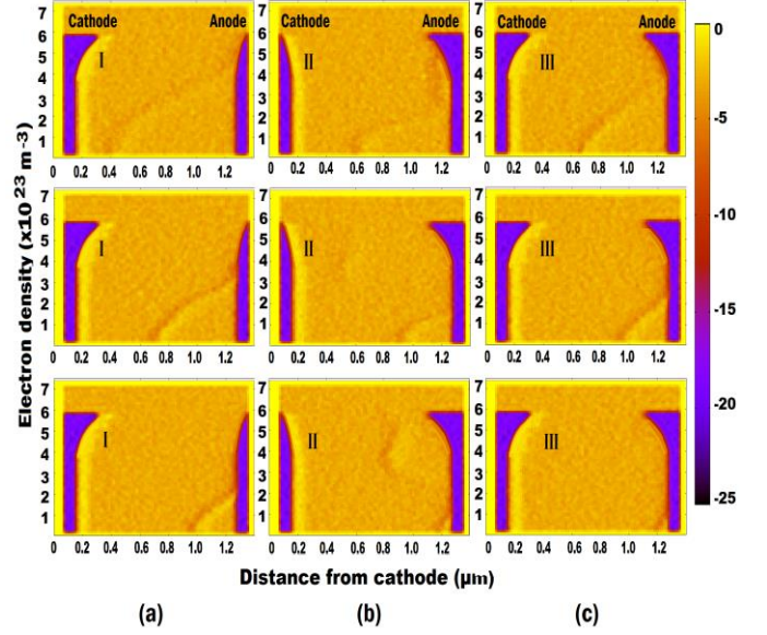
Fig. 6. (I), (II), and (III), shows the electron density (in units of 10^{23}\text{m}^{-3} ) a 1.3 \mu\text{m} -width device under the effect of 1.36 V bias at several instants during the transit in the convex-concave device (a), concave-convex device (b) and concave-concave device (c). In each device (I) The domain forms at 76.1 ps from the cathode. (II) 2.4 ps later the domain has progressed further towards the anode. (III) after another 2.4 ps. The distortion is remarkable.
