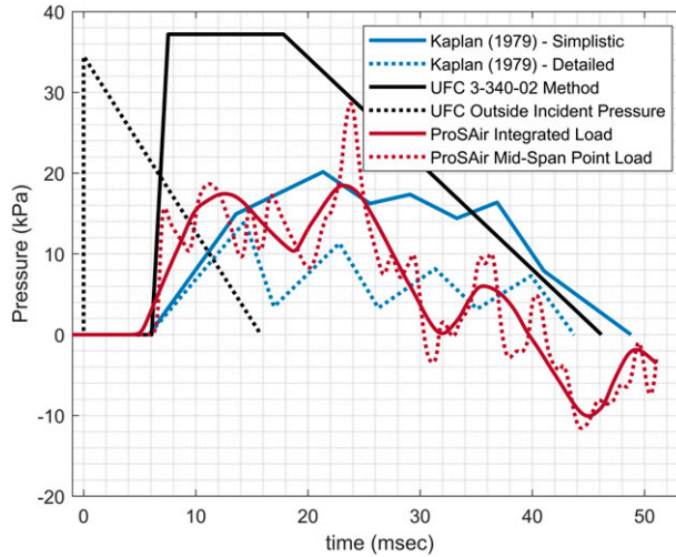
Figure 18. Side wall loadings predictions for Case 3A where W/H = 3/2 , A_o/A_w = 3/16 and L_w/L = 2 .
