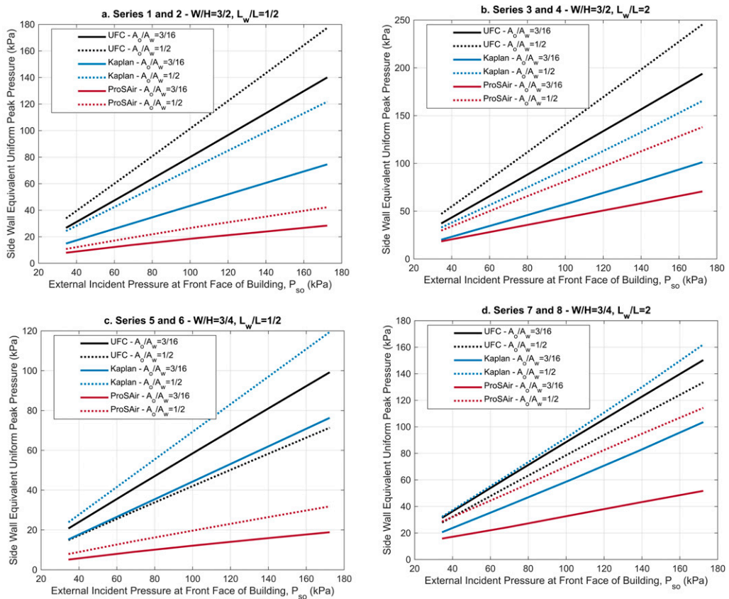
Figure 11. Side wall equivalent uniform peak pressure results for Series 1-8.
