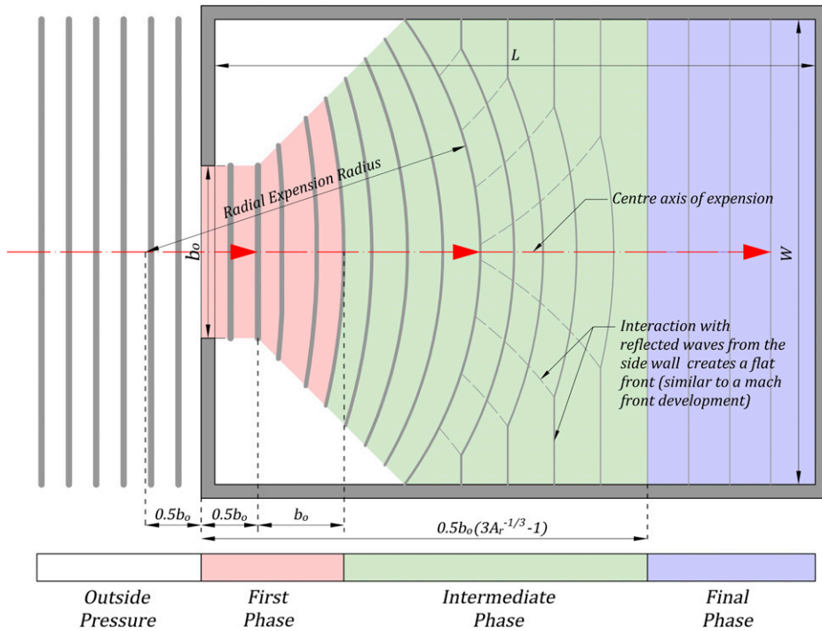
Figure 2. Plan view of Kaplan's (1979) proposed three phases of interior shock wave development as a function of the distance d' travelled from the opening relative to the opening's effective diameter b_o and relative to the total facade area A_r .
