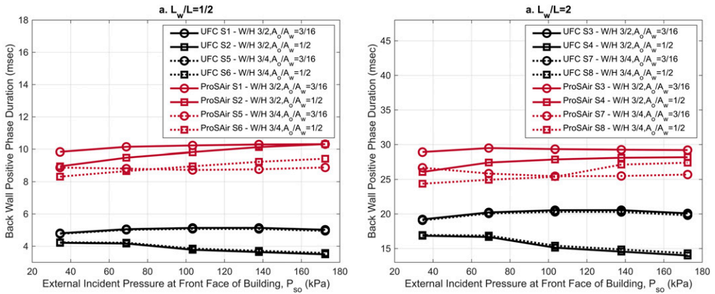
Figure 25. Variation of the predicted back wall positive phase duration with external incident pressure; (left) for Series 1,2,5,6 ( L_w/L = \frac{1}{2} ) and (right) for Series 3,4,7,8 ( L_w/L = 2 ).
