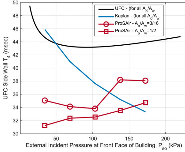
Figure 17. Side wall loading duration T_4 predictions for Series 4-5 where W/H = 3/4 and L_w/L = 2 .
