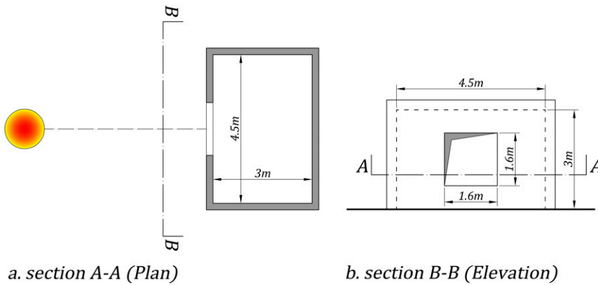
Figure 10. Dimensions of the cuboid structure of Series 1 and 3 with W/H = \frac{3}{2} , A_o/A_w = \frac{3}{16}
