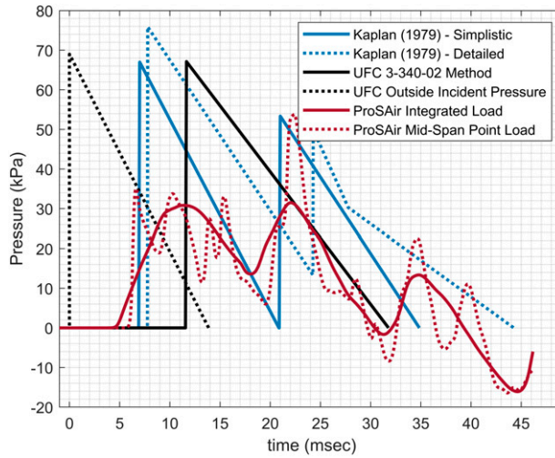
Figure 24. Side wall loadings predictions for Case 3B ( W/H = 3/2 , A_o/A_w = 3/16 and L_w/L = 2 ).
