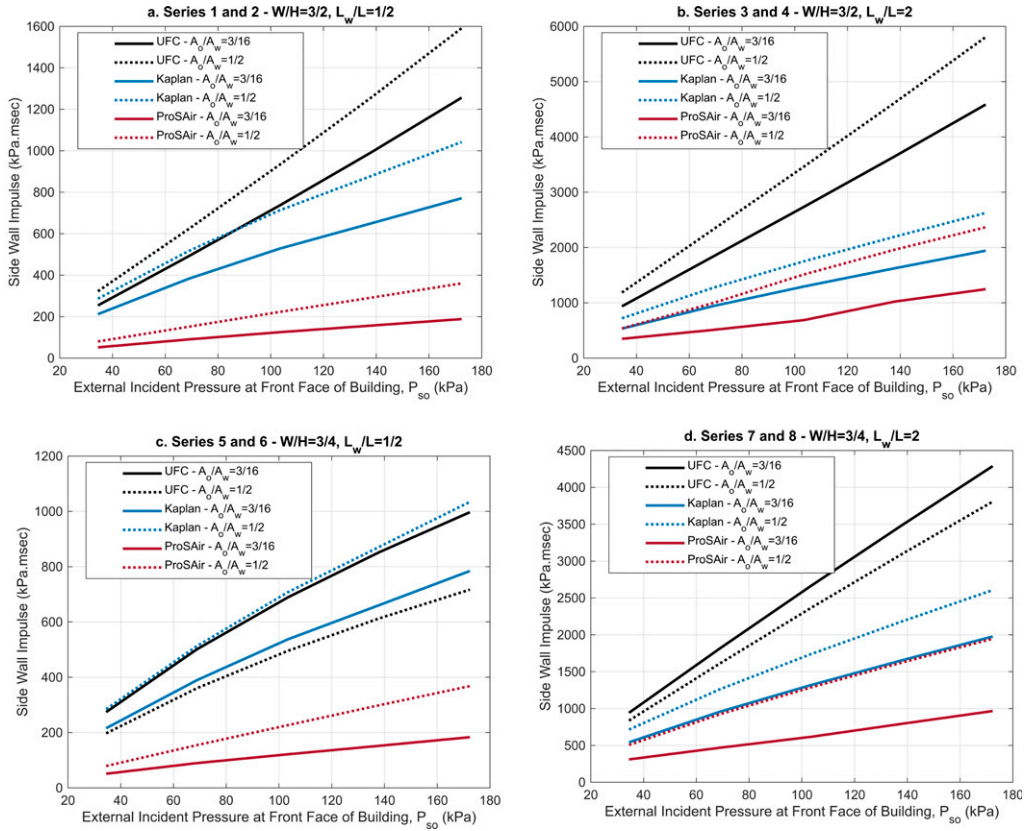
Figure 12. Side wall equivalent uniform first phase impulse results for Series 1-8.
