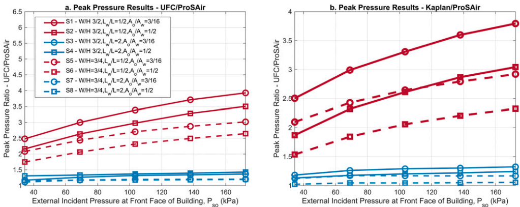
Figure 21. Equivalent uniform peak pressure ratios for Series 1-8; (left) UFC/ProSAir and (right) Kaplan/ProSAir.
