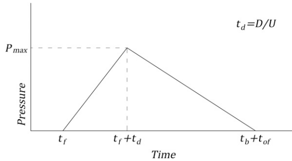
Figure 4. TM 5-1300 – Equivalent uniform pressure loading for a Side Wall span perpendicular to the shock plane, with t_f the wall's shock arrival time, t_d = D/U the resulting time interval to maximum pressure ( D the distance the shock exerts maximum stress, U is the shock velocity), t_b the shock arrival time to the end of the wall, t_{of} = 2i_s/P_{s0} and i_s the incident impulse at the facade.
