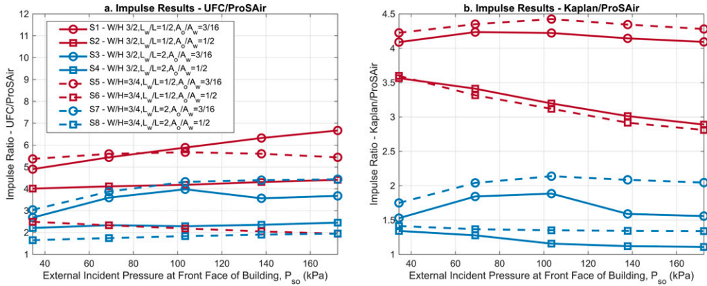
Figure 14. Equivalent uniform impulse ratio for Series 1-8; (left) UFC/ProSAir and (right) Kaplan/ProSAir.
