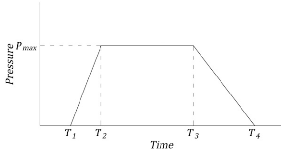
Figure 6. Idealised side wall loading used by the UFC 3-340-02 defined by the four time points ( T_1 , T_2 , T_3 , T_4 ) and maximum plateau pressure P_{max} .
