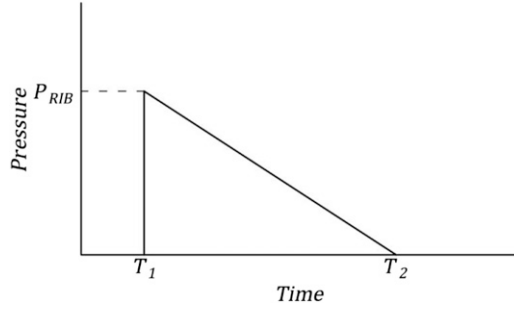
Figure 7. UFC 3-340-02 – Idealised back wall loading defined by two time points T_1 , T_2 , and instantaneous peak reflected pressure P_{RIB} .
