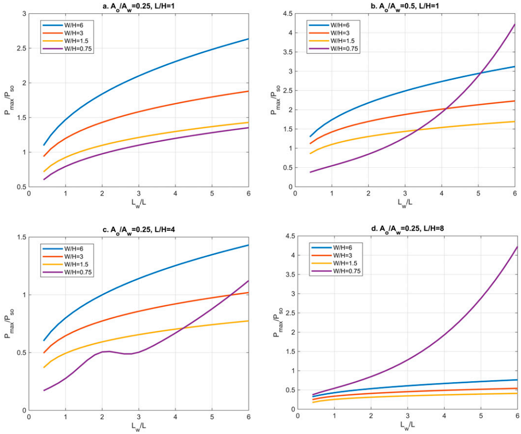
Figure 8. (a-d) Variation of the simplified UFC side wall pressure ratio P_{max}/P_{so} with shock relative wavelength L_w/L for different opening ratios A_o/A_w and building aspect ratios.
