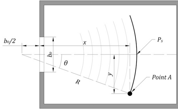
Figure 3. Plan view illustrating the parameters to calculate the off-axis pressure P_{S\theta} at point A as per Equations (2-5) and (2-6).
