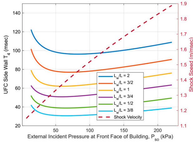
Figure 9. The UFC loading duration T_4 (left-hand axis) and shock speed (dashed, right hand axis) for a side wall with W/H = 3/2 , L/H = 2 versus external incident pressure for various L_w/L ratios.
