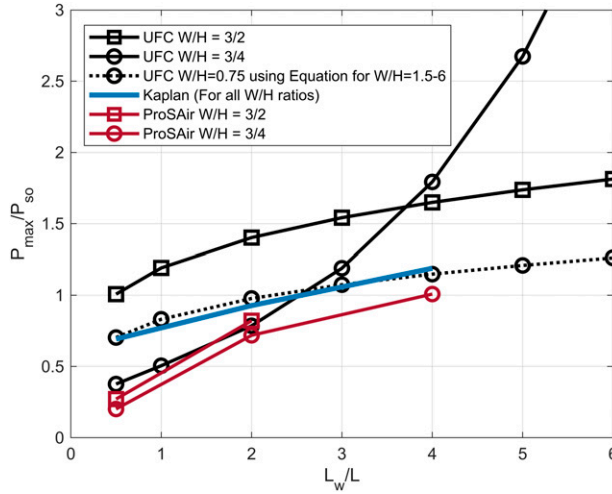
Figure 15. Variation of the UFC side wall P_{max}/P_{SO} with shock relative wavelength L_w/L for A_o/A_w = 0.5 and L/H = 1 .
