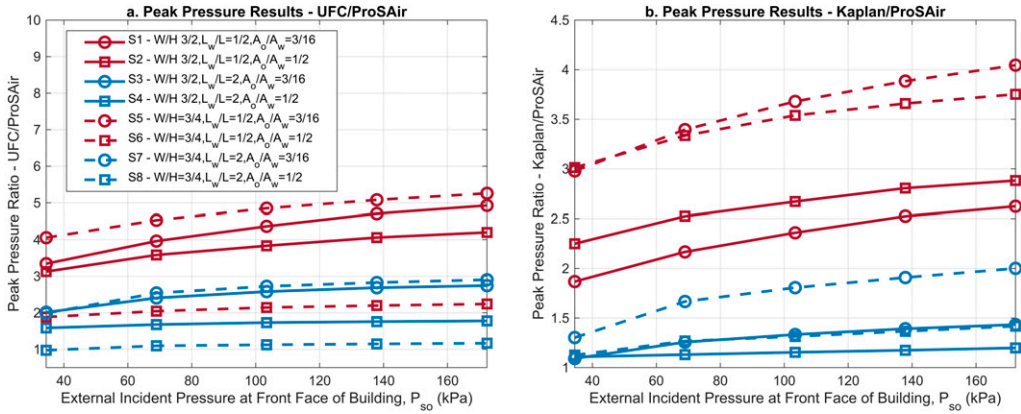
Figure 13. Equivalent uniform peak pressures ratios for Series 1-8; (left) UFC/ProSAir, (right) Kaplan/ProSAir.
