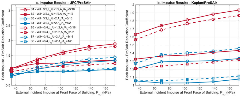
Figure 22. Equivalent uniform impulse ratios for Series 1-8; (left) UFC/ProSAir and (right) Kaplan/ProSAir.
