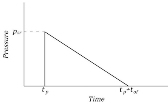
Figure 5. Kaplan's (1979) equivalent uniform pressure loading for the rear wall for instantaneous peak reflected pressure P_{sr} Equation (2-9) and arrival time t_p .
