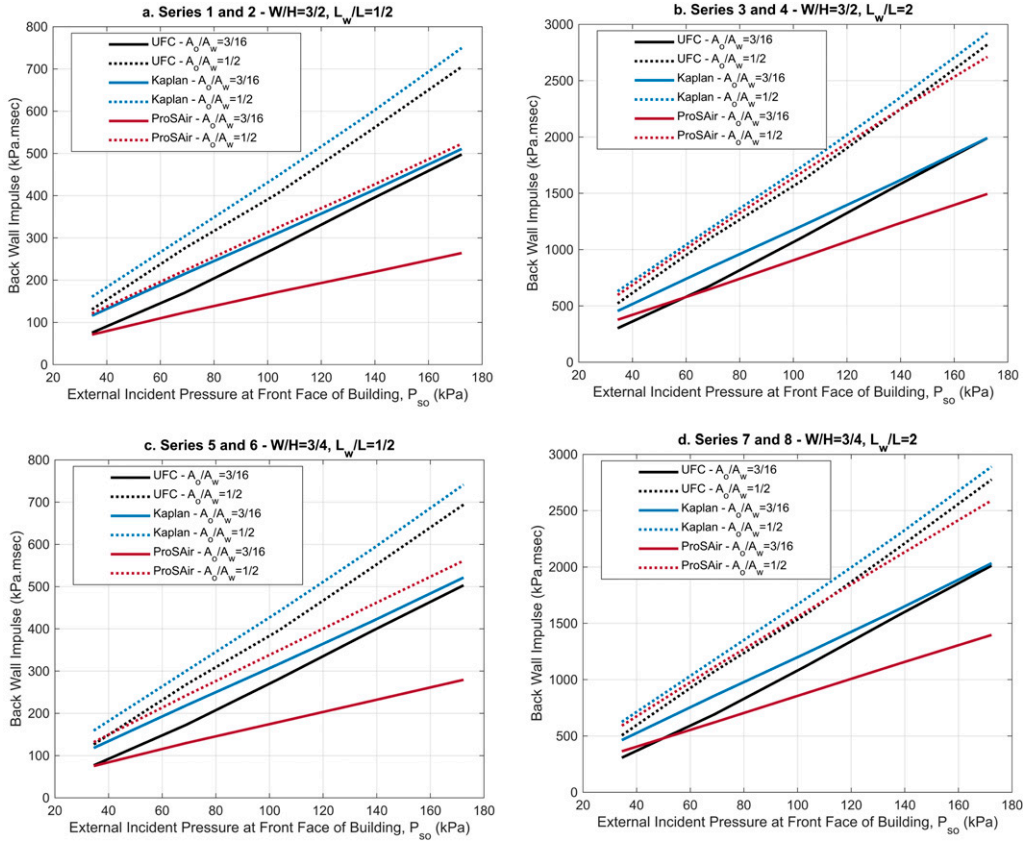
Figure 20. Back wall equivalent uniform first phase impulse results for Series 1-8.
