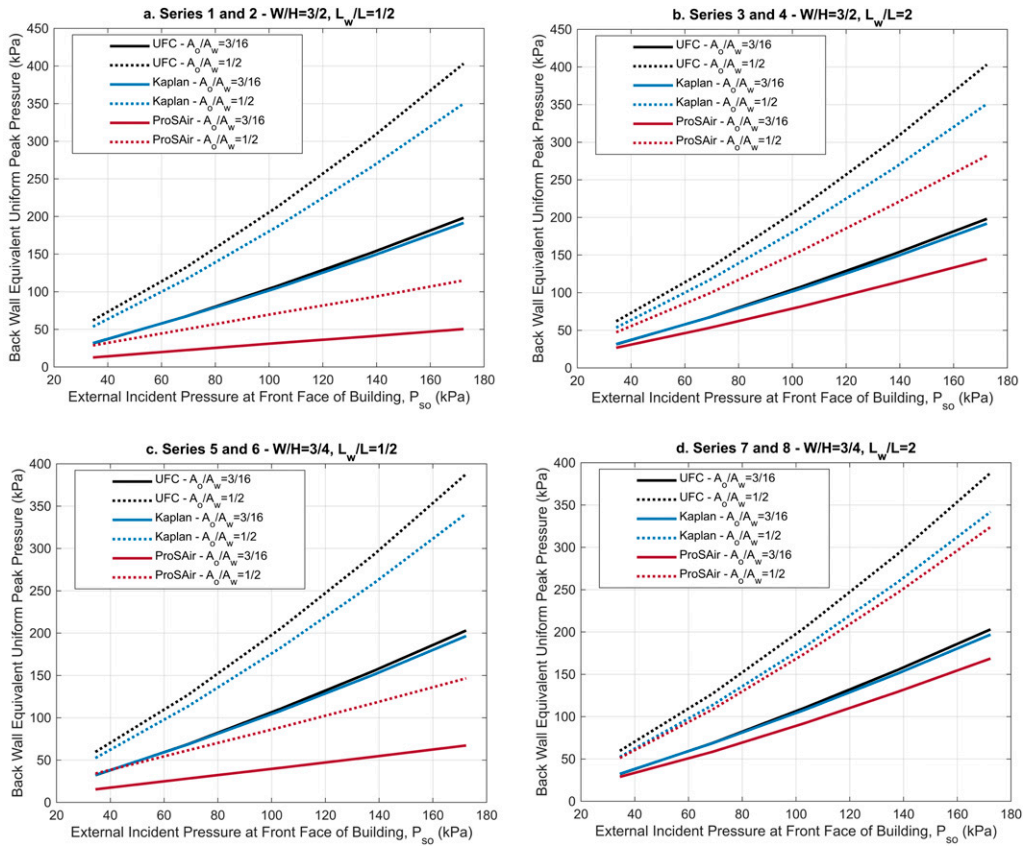
Figure 19. Back wall equivalent uniform peak pressure results for Series 1-8.
