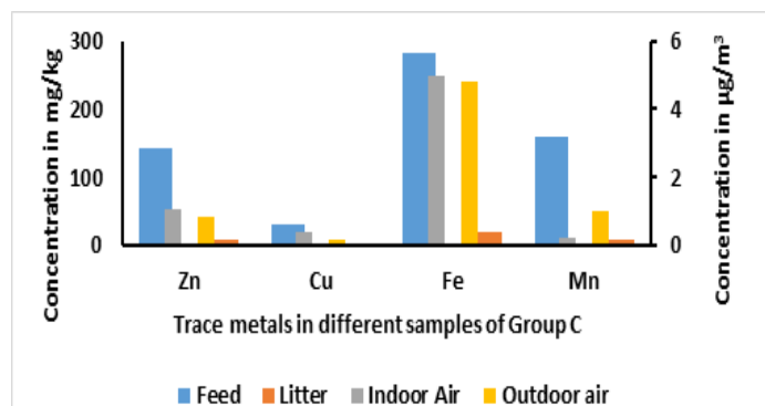
Figure 7: Trace metals in different samples of Group C (Zn: Zinc; Cu: Copper; Fe: Iron; Mn: manganese)
