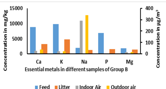
Figure 3: Essential metals in different samples of Group B (Ca: Calcium; K: Potassium; Na: Sodium; P: Phosphorus; Mg: Magnesium)
