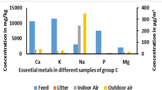
Figure 4: Essential metals in different samples of Group C (Ca: Calcium; K: Potassium; Na: Sodium; P: Phosphorus; Mg: Magnesium)
