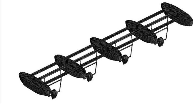
Fig 2. Pentamaran mesh visualization
