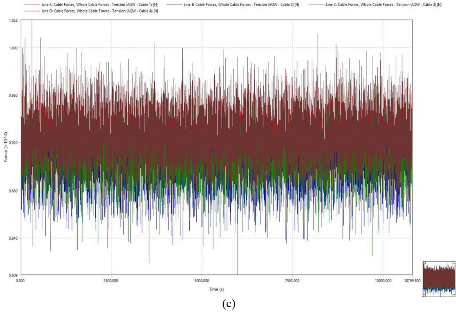
Fig 7. Maximum cable tension for pentamaran FPV with turbine: (a) 0 dg; (b) 90 dg; (c) 45 dg
