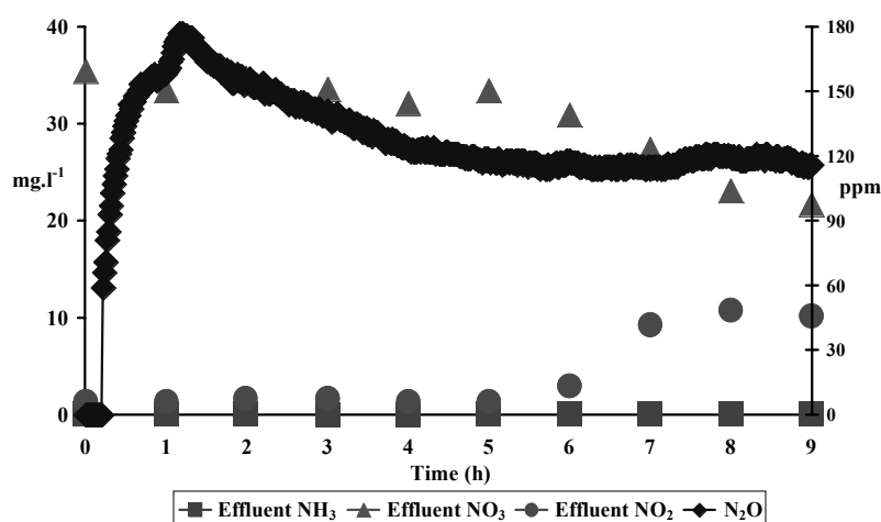
Figure 10: Sodium azide shock load at 75 % of reported minimum inhibitory concentration
