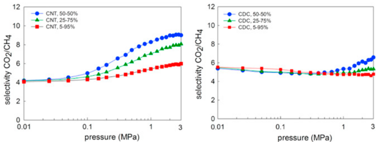
Figure 14. Selectivity of CO 2 :CH 4 gases in CNT and SiC-DC at various compositions [130]. ‘Reprinted from Ref. [130], with permission from Elsevier’.
