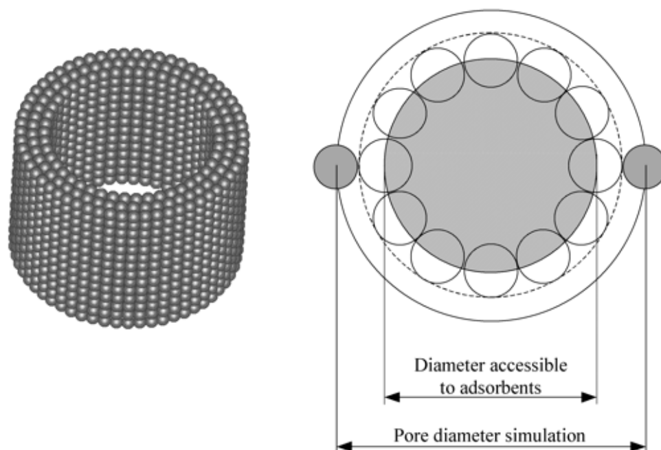
Figure 6. Yun et al.’s model of MCM-41, with the structure composed of only oxygen atoms [89]. ‘Reprinted (adapted) with permission from [89]. Copyright 2002 American Chemical Society’.
