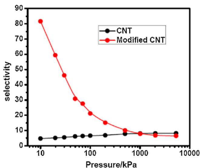
Figure 16. Simulated results for CO 2 /CH 4 selectivity on modified and unmodified CNT [44]. ‘Reprinted from Ref. [44], with permission from Elsevier’.
