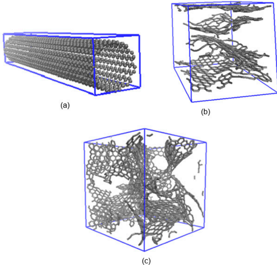
Figure 13. Simulation input for the structural framework of (a) CNT, (b) ACF-15, and (c) SiC-DC [130]. ‘Reprinted from Ref. [130], with permission from Elsevier’.
