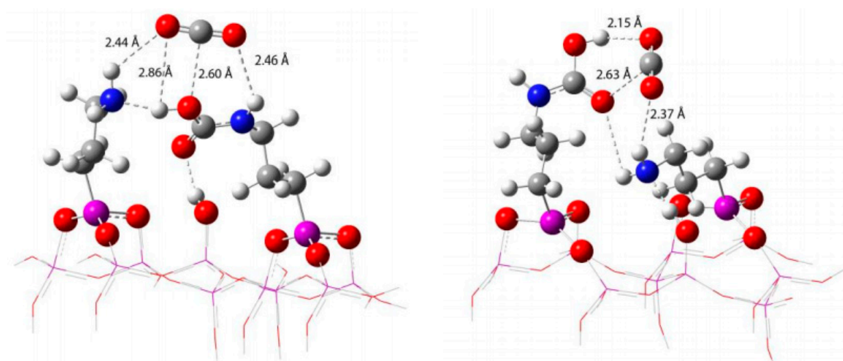
Figure 9. Interaction of physisorbed \text{CO}_2 with carbamic acid and non-reacted \text{NH}_2 moieties [103]. 'Reprinted (adapted) with permission from [103]. Copyright 2017 Elsevier B.V. All rights reserved'.
