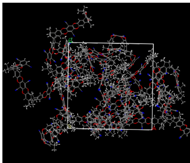
Figure 18. Polymer membrane unit cell processed through amorphous cell builder [140]. ‘Reprinted from Ref. [140], with permission from Taylor & Francis Ltd.’.
