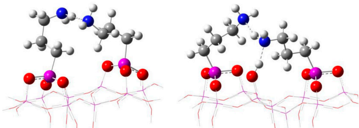
Figure 8. APTES-modified silica surface post-DFT geometric optimization [103]. ‘Reprinted (adapted) with permission from [103]. Copyright 2017 Elsevier B.V. All rights reserved’.
