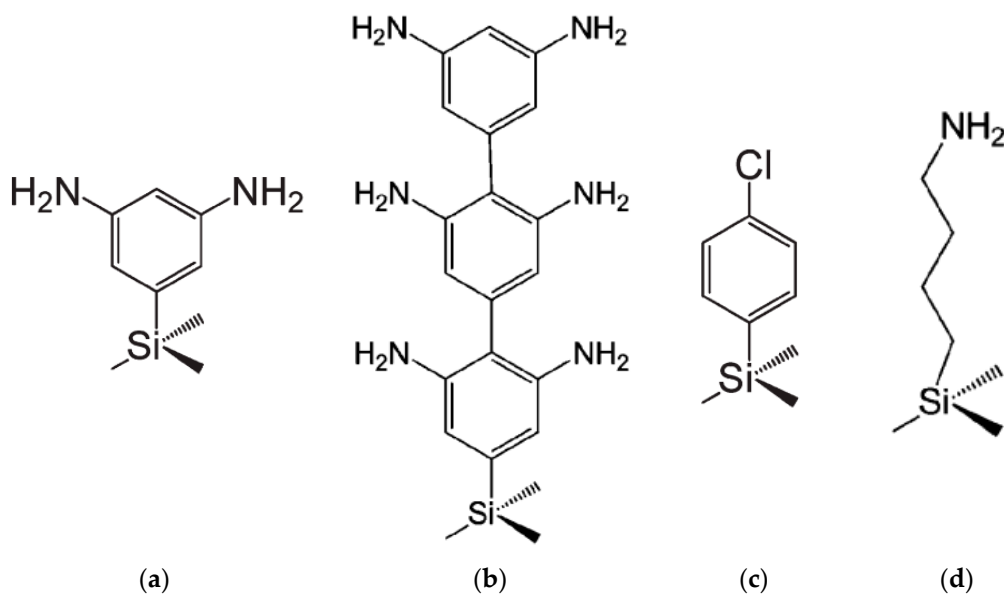
Figure 12. Structure of (a) Diaminophenyl with silanol bond, (b) Hexaminoterphenyl, (c) Chlorophenyl, (d) Butylamine.
