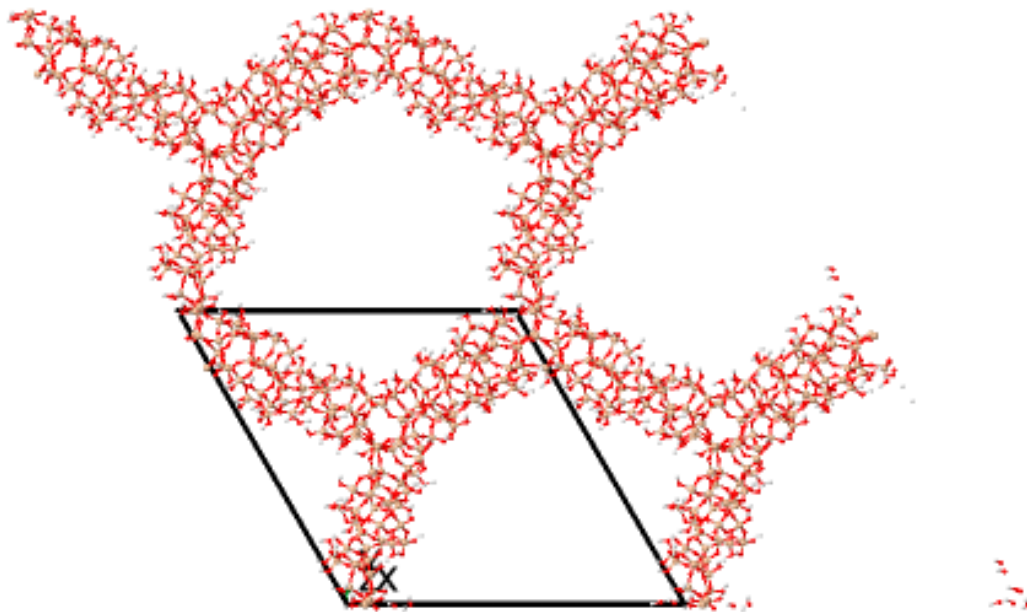
Figure 2. Mesoporous silica MCM-41 Unit Cell and periodic structure visualization for GCMC calculations [56]. ‘Reprinted from Ref. [56]’.
