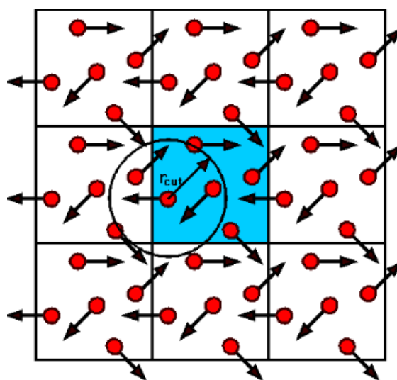
Figure 3. Periodic boundary conditions as applied to component translation moves [58]. The red circle represents an example molecule, while the arrows are the possible movements as implemented by GCMC software within the periodic boundary (In blue). ‘Reprinted from Ref. [58]’.
