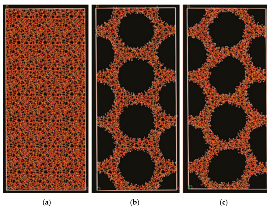
Figure 4. Steps in the construction of the MCM-41 model—(a) Amorphous Silica. (b) Carving Cylindrical Pores. (c) Post-geometric optimization by MM [31]. ‘Reprinted (adapted) with permission from [31]. Copyright 2008 American Chemical Society’.
