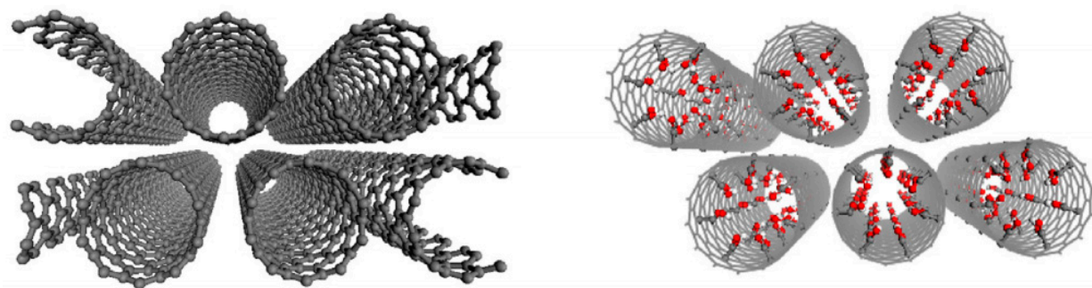
Figure 15. Simulation structure for unmodified and COOH-surface-modified CNT [44]. The red spheres represent Oxygen, white represents hydrogen, and grey represent carbon. ‘Reprinted from Ref. [44], with permission from Elsevier’.
