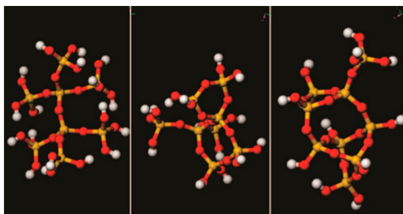
Figure 5. Three different Amorphous Silica clusters used for ESP partial charge determination [31]. ‘Reprinted (adapted) with permission from [31]. Copyright 2008 American Chemical Society’.
