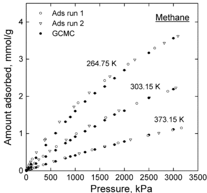
Figure 7. Comparison of experimental and simulated Methane pure component Isotherms [89]. 'Reprinted (adapted) with permission from [89]. Copyright 2002 American Chemical Society'.
