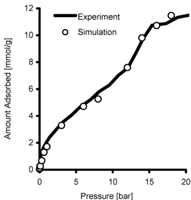
Figure 11. CO 2 Isotherm on Aminopropyl-modified MCM-41. 263K, AP:Si = 0.1. ‘Reproduced with permission from Springer Nature’ [35].
