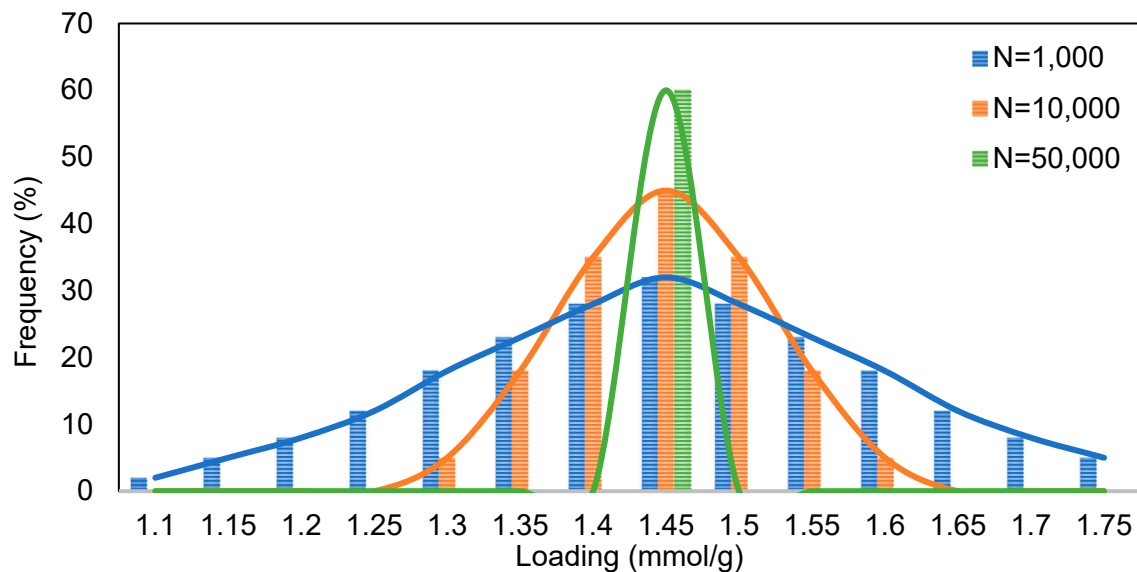
Figure 1. Monte Carlo probability distribution of a hypothetical adsorbent loading based on the frequency of sampling represented by N. The line follows the trend of each probability distribution.
