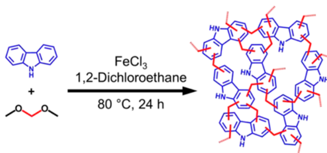
Figure 17. HCP synthesis via knitting or external crosslinking with functional group to provide enhanced adsorption performance [137]. 'Reprinted from Ref. [137]'.
