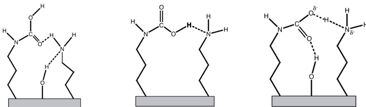
Figure 10. Structures of species formed by carbamic acid interaction with adsorbent surface and neighbouring molecules [108]. 'Reprinted (adapted) with permission from [108]. Copyright 2017 American Chemical Society'.
