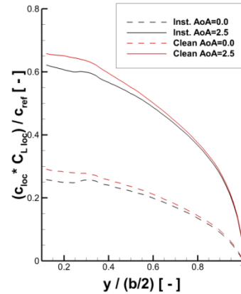
Figure 13 The spanwise distribution of non-dimensional lift coefficient ( C_{L loc} C_{L loc} / C_{ref} ) for CRM with (installed) and without (clean) engine at AoA_{A/C} = 0.0^\circ and AoA_{A/C} = 2.5^\circ ; Re = 45 \times 10^6 ; M_\infty = 0.82
