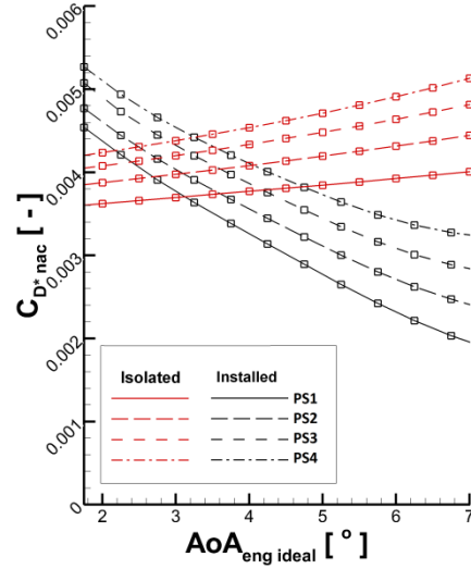
Figure 30 Modified engine drag ( C_{D^* nac} ) as function of engine ideal incidence ( AoA_{eng,ideal} ) for the baseline engine in isolation and under the wing in baseline position (C3) for a range of power settings from PS1 to PS4; Re = 45 \times 10^6 ; M = 0.82 ;
