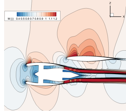
Figure 11 Contours of Mach Number at the spanwise cross-section through the engine axis in position C3 in power setting “PS1”; AoA_{A/C} = 2.5^\circ ; Re = 45 \times 10^6 ; M_\infty = 0.82
