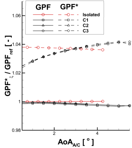
Figure 28 Specific gross propulsive force ( GPF_\xi ) and modified gross propulsive force ( GPF_\xi^* ) for isolated nacelle compared with baseline engine (PS1) in three vertical positions (C1, 'C2' and C3); Re = 45 \times 10^6 ; M = 0.82 ;
