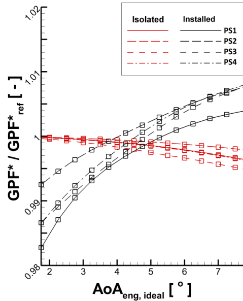
Figure 34 Non-dimensionalised modified gross propulsive force ( GPF^* / GPF^*_{ref} ) for baseline configuration (C3) in four engine power settings compared with isolated engine; Re = 45 \times 10^6 ; M = 0.82
