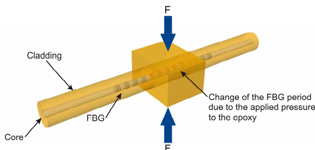
Fig. 1: FBG embedded within epoxy material. F: force.
