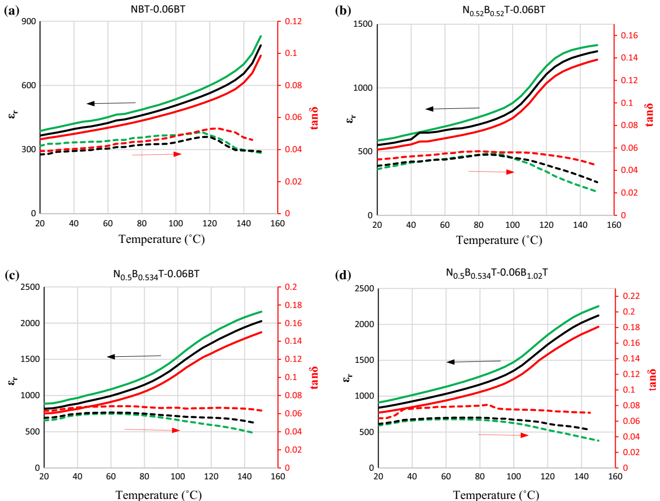
Figure 3 Relative permittivity ( \epsilon_r ) and loss tangent ( \tan\delta ) versus temperature for a NBT-0.06BT, b N_{0.52}B_{0.52}T-0.06BT , c N_{0.5}B_{0.534}T-0.06BT , and d N_{0.5}B_{0.534}T-0.06B_{1.02}T at three
