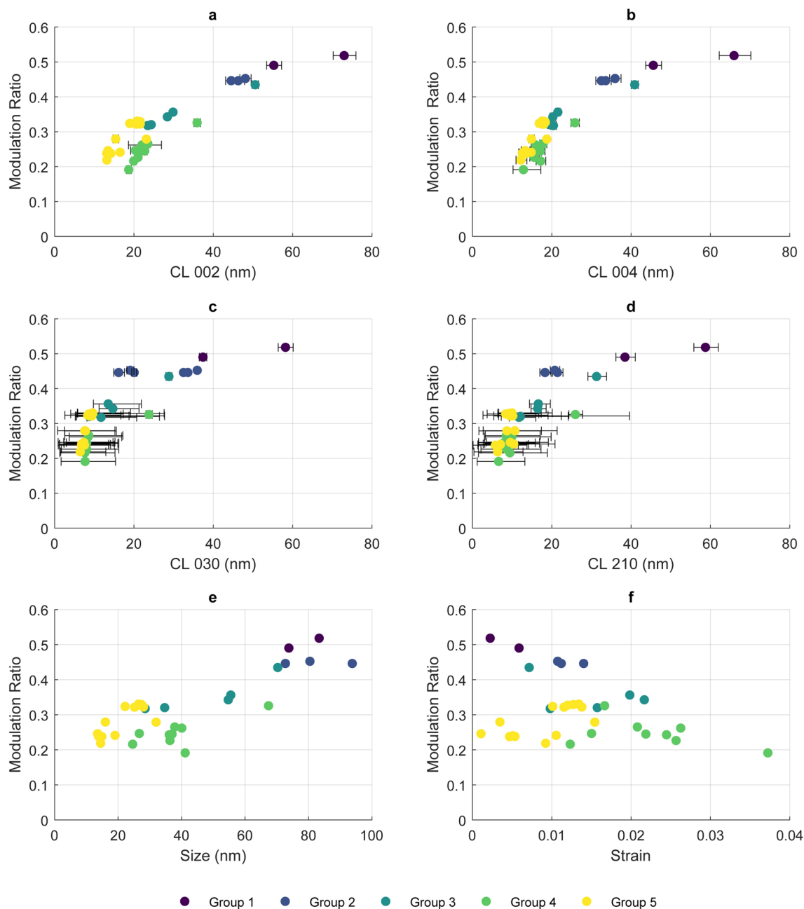
Figure 3. Relationship between MR and (a) 002 CL and MR, (b) 004 CL, (c) 030 CL, (d) 210 CL, (e) size (L) in \langle 00\ell \rangle and (f) strain ( \epsilon ) in \langle 00\ell \rangle . Error bars represent peak fitting errors.
