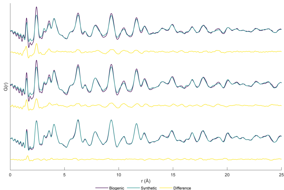
Figure 2. Comparison of biogenic and synthetic samples (and difference plots below) from bottom to top: mesoplodan rostrum (90.80 Ash%, 10.37 wt% \text{CO}_3^{2-} ) and synthetic (7.52 wt% \text{CO}_3^{2-} ), bovine (69.29 Ash%, 7.00 wt% \text{CO}_3^{2-} ) and synthetic (8.12 wt% \text{CO}_3^{2-} ), cervine antler (55.63 Ash%, 5.43 wt% \text{CO}_3^{2-} ) and synthetic (5.83 wt% \text{CO}_3^{2-} ).
