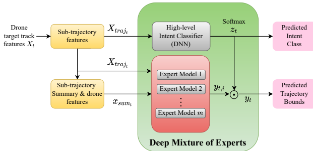
Fig. 2. Deep Mixture of Experts Network for Drone Intent Classification and Regression Prediction
