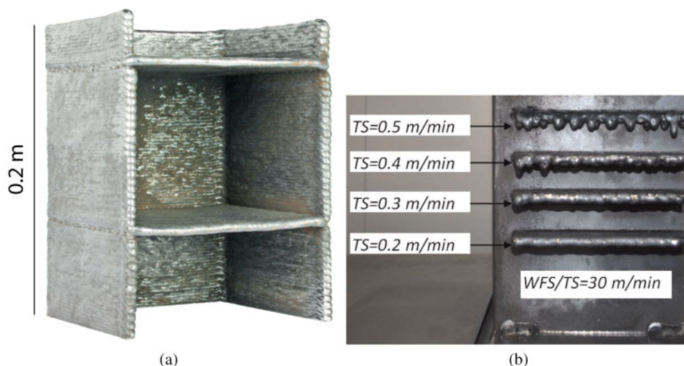
a box structure deposited vertically; b horizontal features deposited without supports 26
