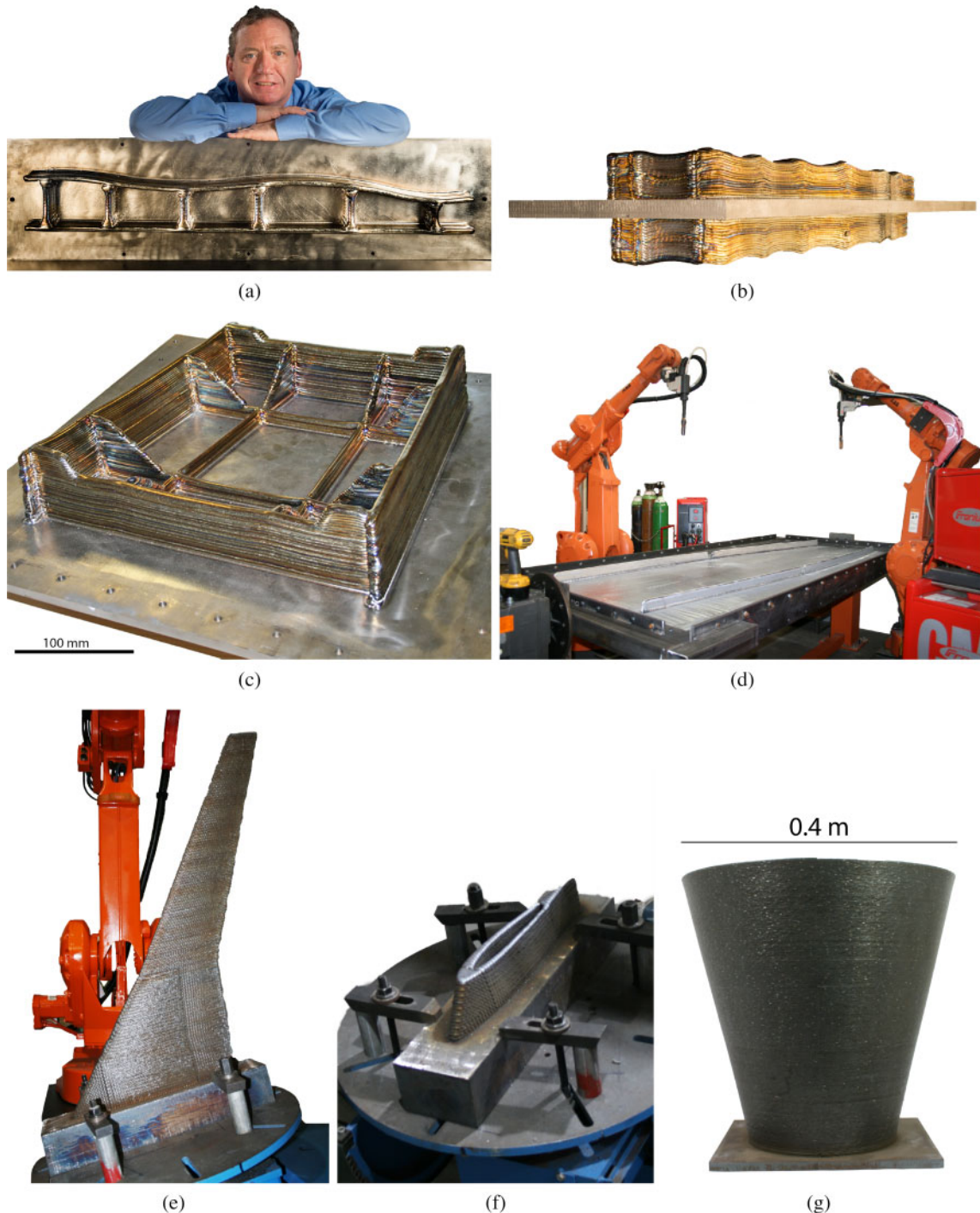
a 1.2 m Ti-6Al-4V wing spar built for BAE Systems; 15 process: PAWWAAM; b side view (please note two-component built back to back; courtesy of BAE Systems 15 ); c 24 kg Ti-6Al-4V external landing gear assembly (process: PAWWAAM); d 2.5 m aluminium wing spar (process: Fronius CMT Advanced 11 WAAM); e high strength steel wing model for wind tunnel testing (process: Fronius CMT 11 WAAM); f particular of hollow structure; g mild steel truncated cone (process: Fronius CMT 11 WAAM)
