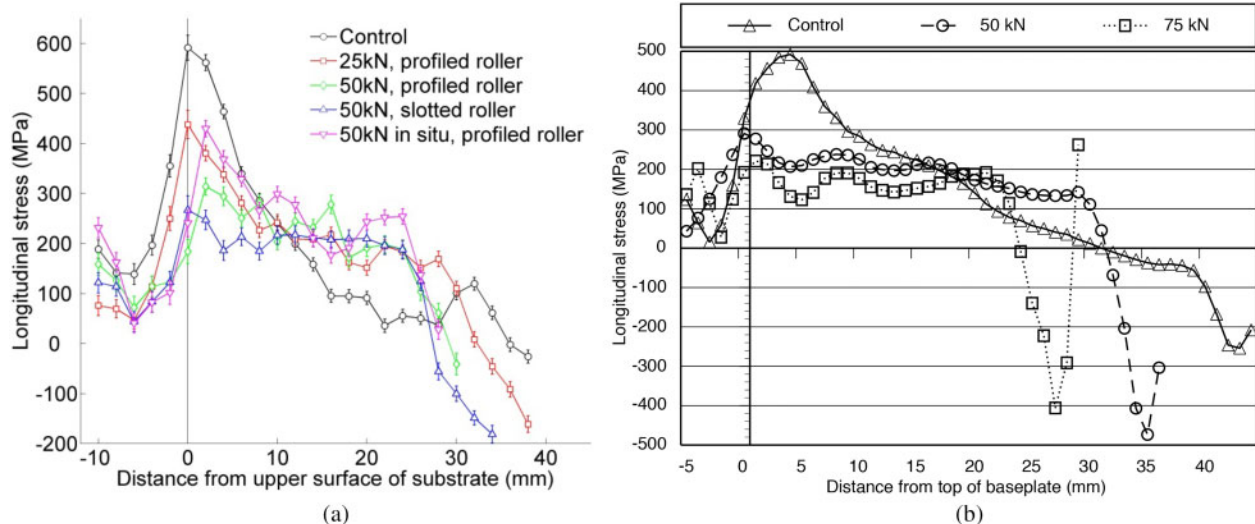
a residual stress reduction in steel WAAM components; 19 b residual stress reduction in Ti-6Al-4V WAAM components 25,28 5 Effect of high pressure interpass rolling on residual stress in longitudinal direction for WAAM components
