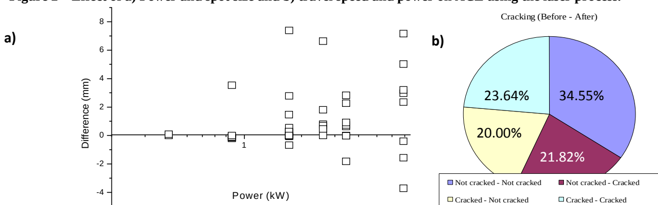
Figure 3 - A) the difference after PWHT of total crack length in laser welds 0.7 and 1.71mm, and b) changes in cracking before and after PWHT
