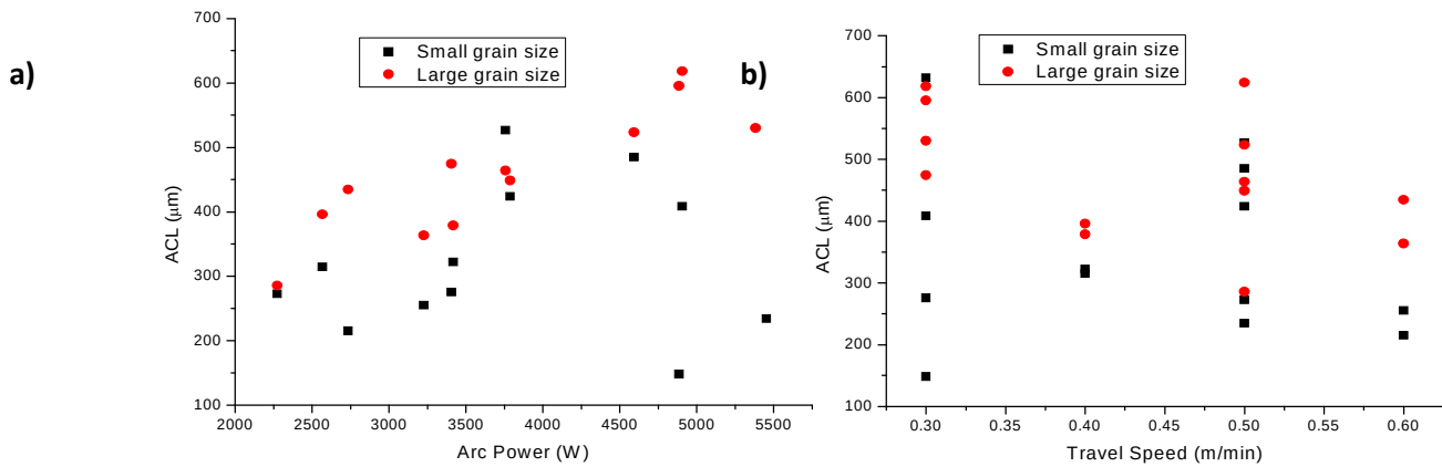
Figure 1 – Effect of a) arc power and b) travel speed on ACL using the CMT process.
