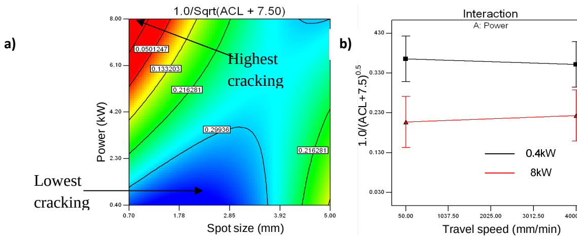
Figure 2 – Effect of a) Power and spot size and b) travel speed and power on ACL using the laser process.
