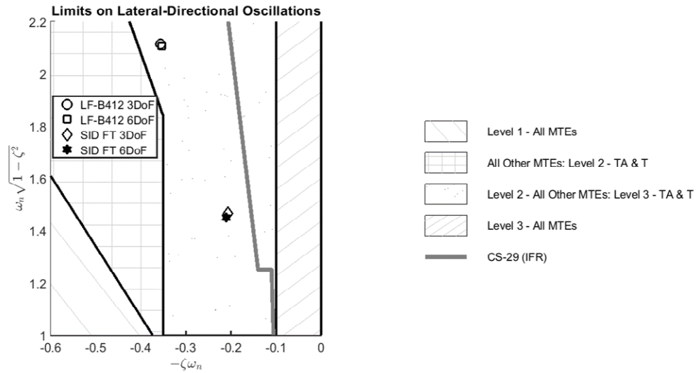
Fig. 10. Comparison of LDO characteristics; SID estimates from flight and predictions from the linearized F-B412.
