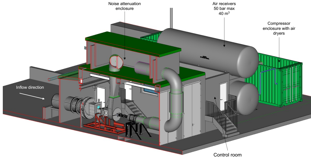
Figure 1 General layout of supersonic intake distortion test rig integrated within test cell
