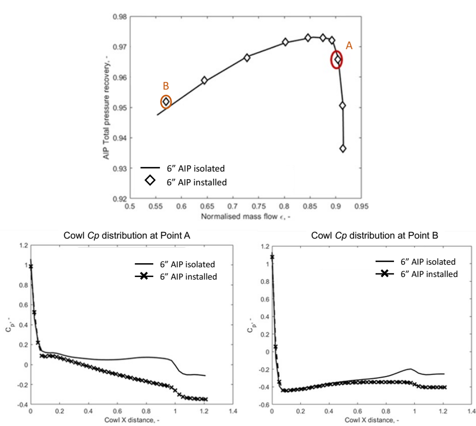
Figure 10 Intake characteristic compared to the uninstalled case across the range of flow ratios at free stream Mach number M_0=1.6 (top). Cowl C_p distribution at symmetry plane in relation to the uninstalled case at Point A, \epsilon=0.904 (bottom-left) and Point B, \epsilon=0.57 (bottom-right)
