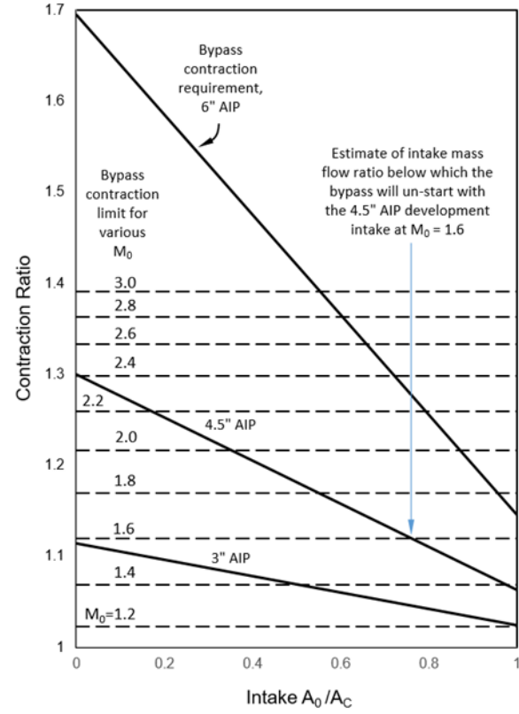
Figure 6 Ideal bypass contraction limit for starting compared to the bypass flow contraction requirement for the three development intakes across a range of mass flow ratios
