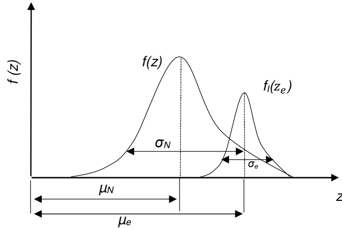
Figure 2: Extreme value distribution of pit depths. f(z) is the probability density function for all the pits and f_I(z_e) is the extreme probability density function
