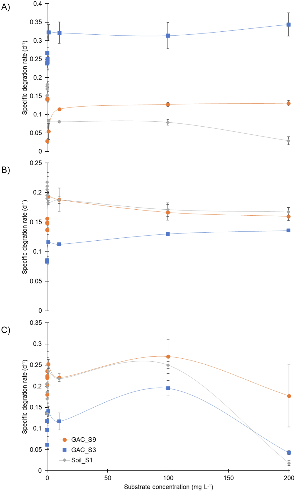
Fig. 5. Specific degradation rate per over different substrate concentrations for each isolate and substrate media used. A) AMPA supplemented MSM, B) LB, C) Raw Untreated water.
