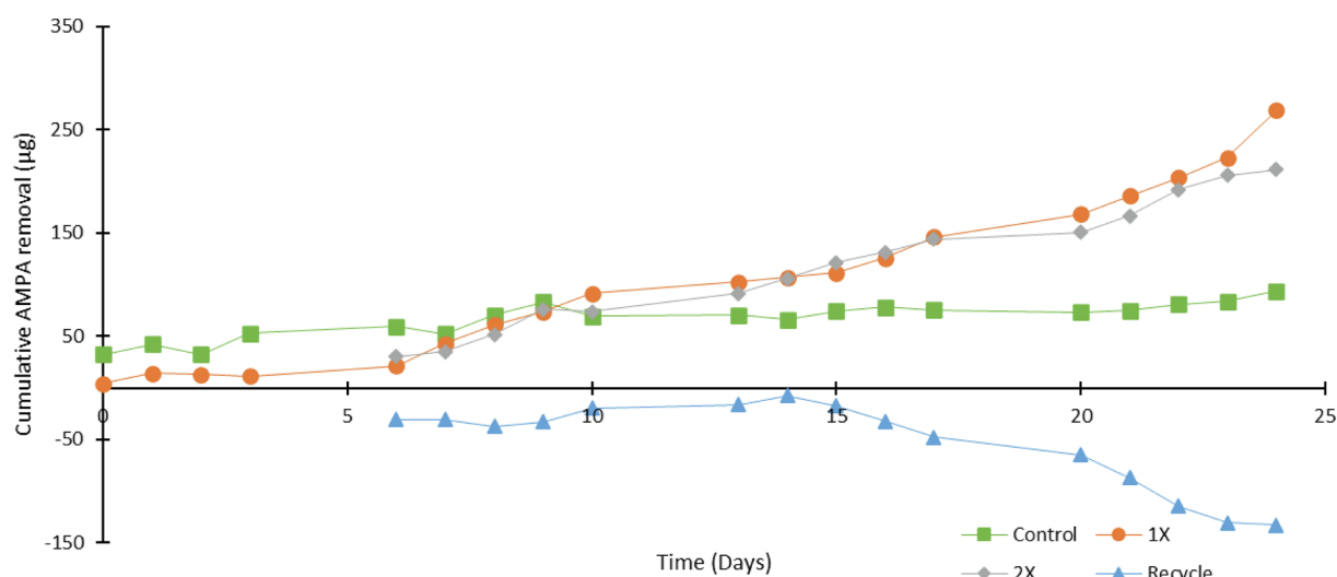
Fig. 6. Cumulative AMPA removal (g) over the duration of the pilot scale study.
