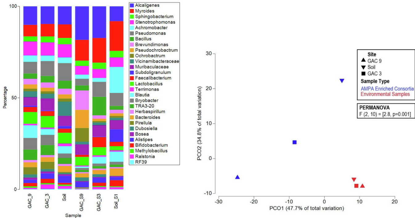
Fig. 2. A) Community of bacteria in the isolates and environmental samples at genus level showing the relative abundance of 16 s rRNA gene copies limited to the top 30. B) Principal ordinate analysis (PCoA) plot of weighted UniFrac distance of the environment.
