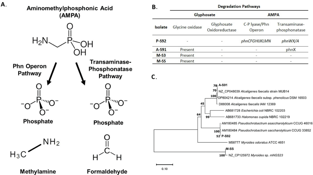
Fig. 3. A) Enzymatic degradation pathways of (Aminomethyl)phosphonic Acid – AMPA. B) Degradation pathways present for each of the isolates. C) Phylogenetic tree of each of the isolate.
