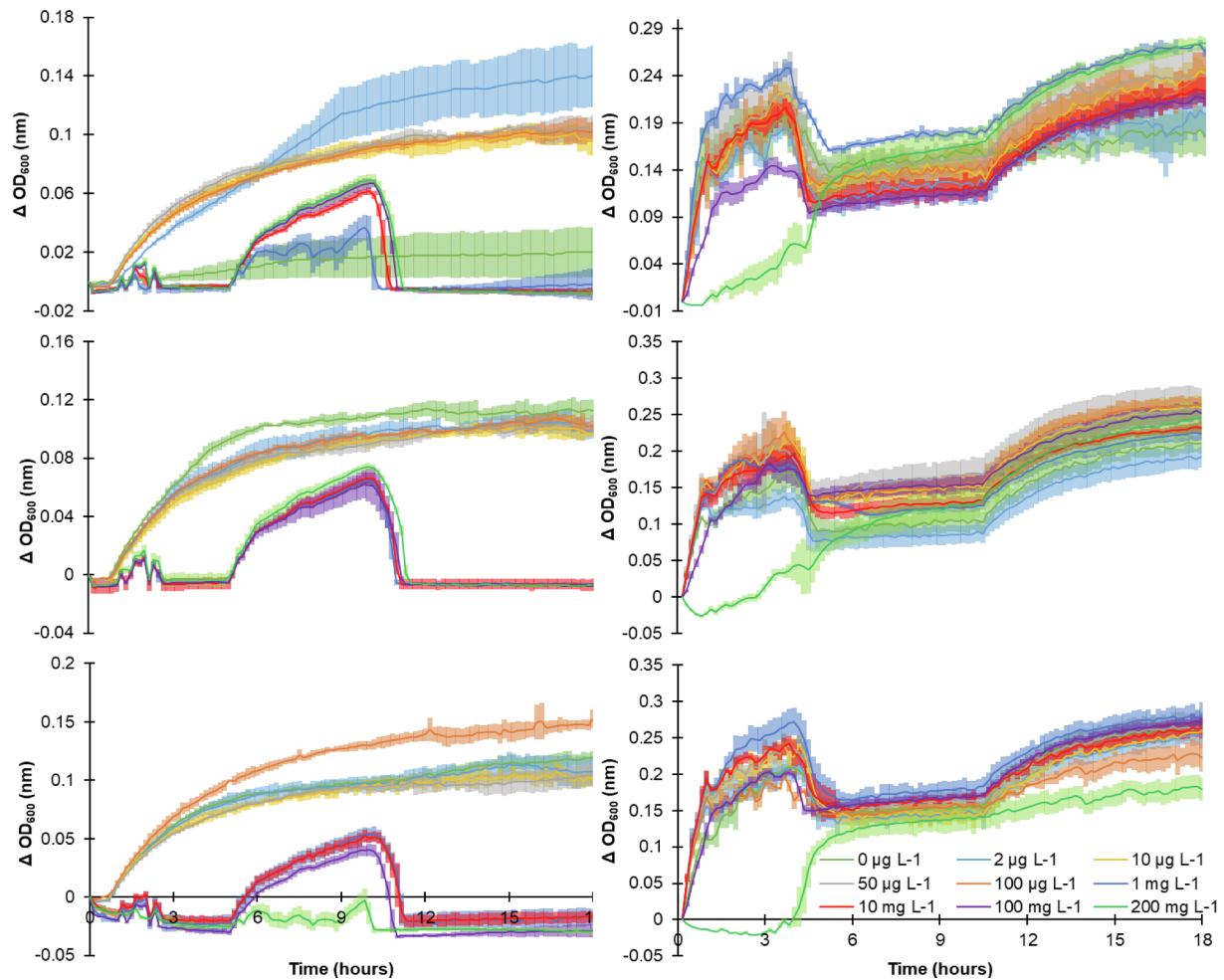
Fig. 4. \Delta OD_{600} showing the growth of each of the isolates in minimal media and untreated water, with concentrations of 0 \mu\text{g/L} , 2 \mu\text{g/L} , 10 \mu\text{g/L} , 50 \mu\text{g/L} , 100 \mu\text{g/L} , 1 mg/L, 10 mg/L, 100 mg/L, 200 mg/L. 1. A. GAC.S9 MSM B. GAC.S9 Untreated water, C. GAC.S3 MSM D. GAC.S3 Untreated water, E. Soil.S1 MSM F. Soil.S1 Untreated water. Data obtained every 10 min with measurements represented as averages of 5 replicates \pm standard deviation.
