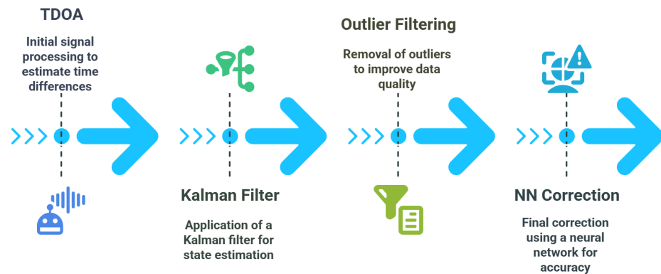
Figure 4. Signal processing pipeline for position estimation.
