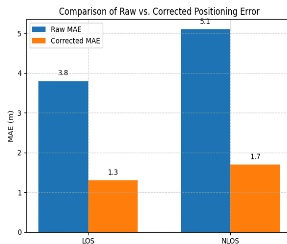
Figure 10. Visual comparison of raw versus corrected position estimation error under LOS and NLOS conditions.
