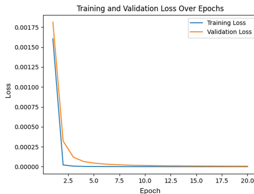
Figure 6. Convergence of training and validation loss over epochs. The y-axis represents the loss value, and the x-axis shows the number of epochs.
