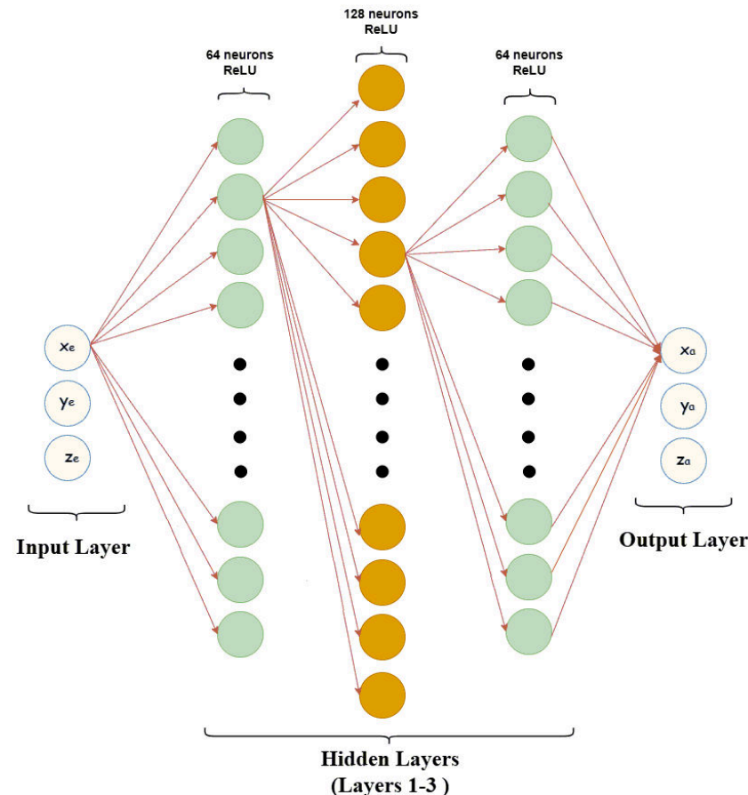
Figure 5. Diagram of the neural network architecture.
