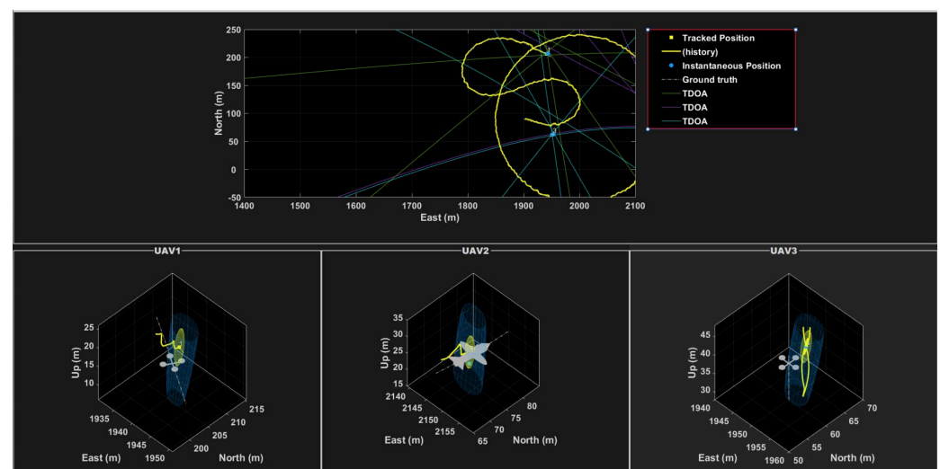
Figure 3. The 5G-enabled urban UAV positioning scenarios. The simulation includes effects such as path loss, multipath fading, and receiver noise to improve practical realism.
