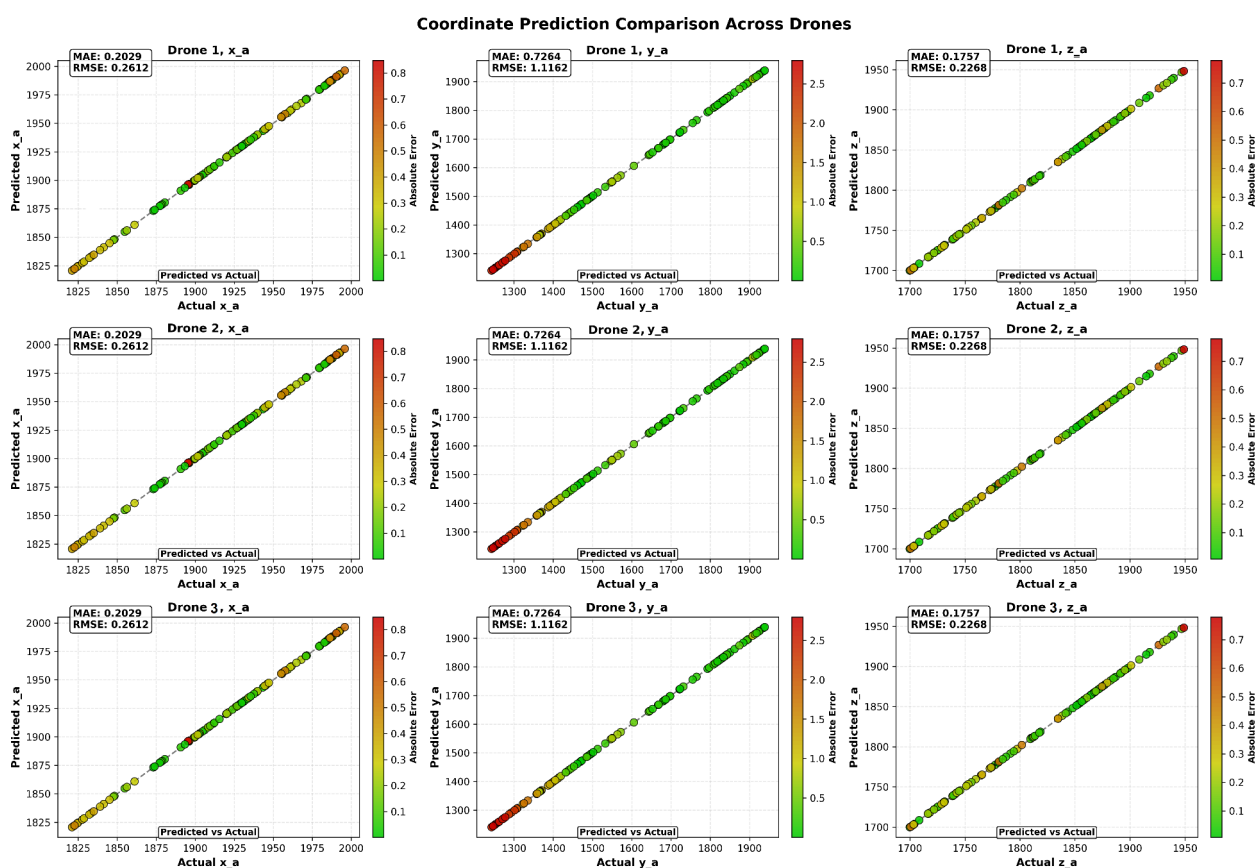
Figure 7. Scatter plots of the predicted vs. actual positions for UAVs 1–3 across X, Y, and Z dimensions. Marker color indicates absolute error (green = low, red = high).
