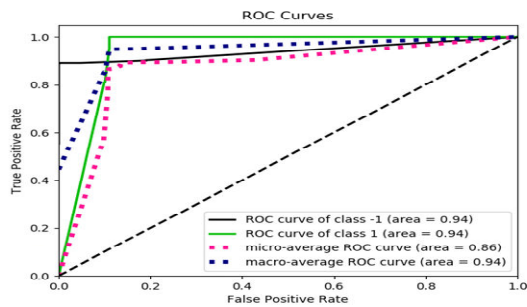
Figure 12. ROC for 5RV1
