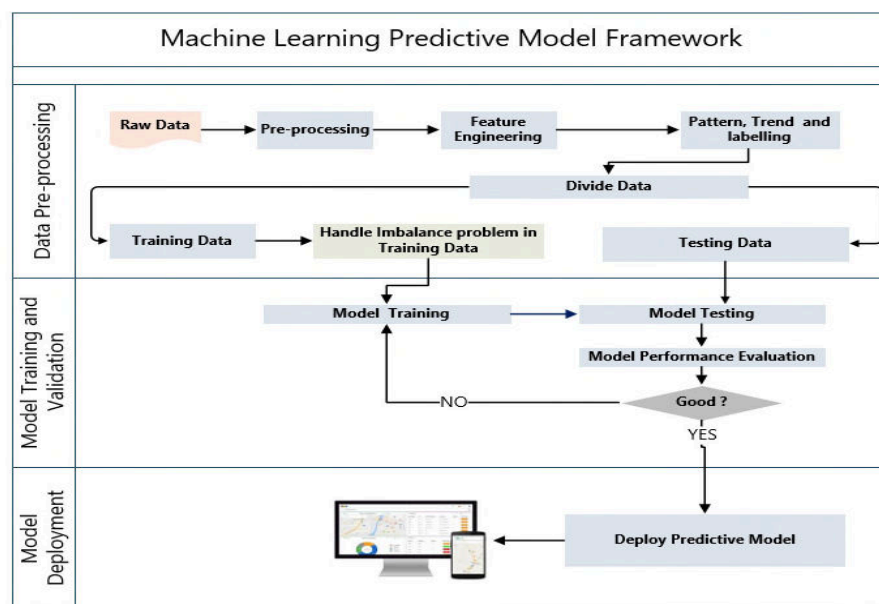
Figure 2. The pipeline for developing predictive model using imbalanced dataset
