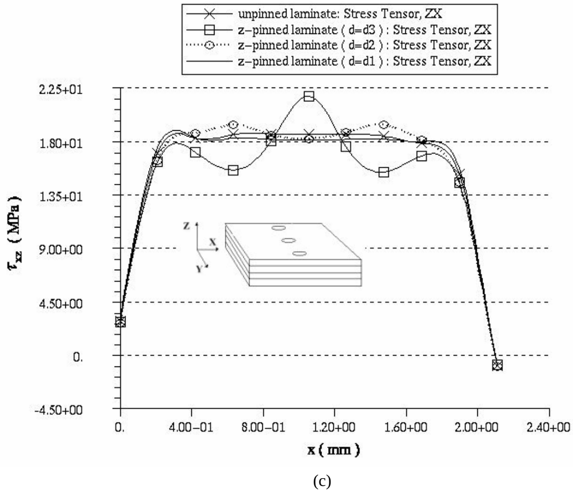
Fig. 7 FE results of \tau_{xz} stress distribution for [45, -45]_s angle-ply laminate: (a) through-the-thickness variation (along z -axis); (b) from inside plate to the free-edge ( y -axis); (c) along the free-edge ( x -axis).
