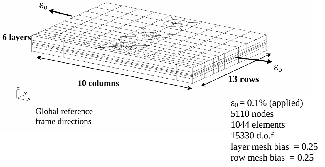
Fig. 2 (b) Finite element model of \frac{1}{4} z-pinned cross-ply laminate, [0, 90] , under applied micro-strain \epsilon_0=0.1\% .
