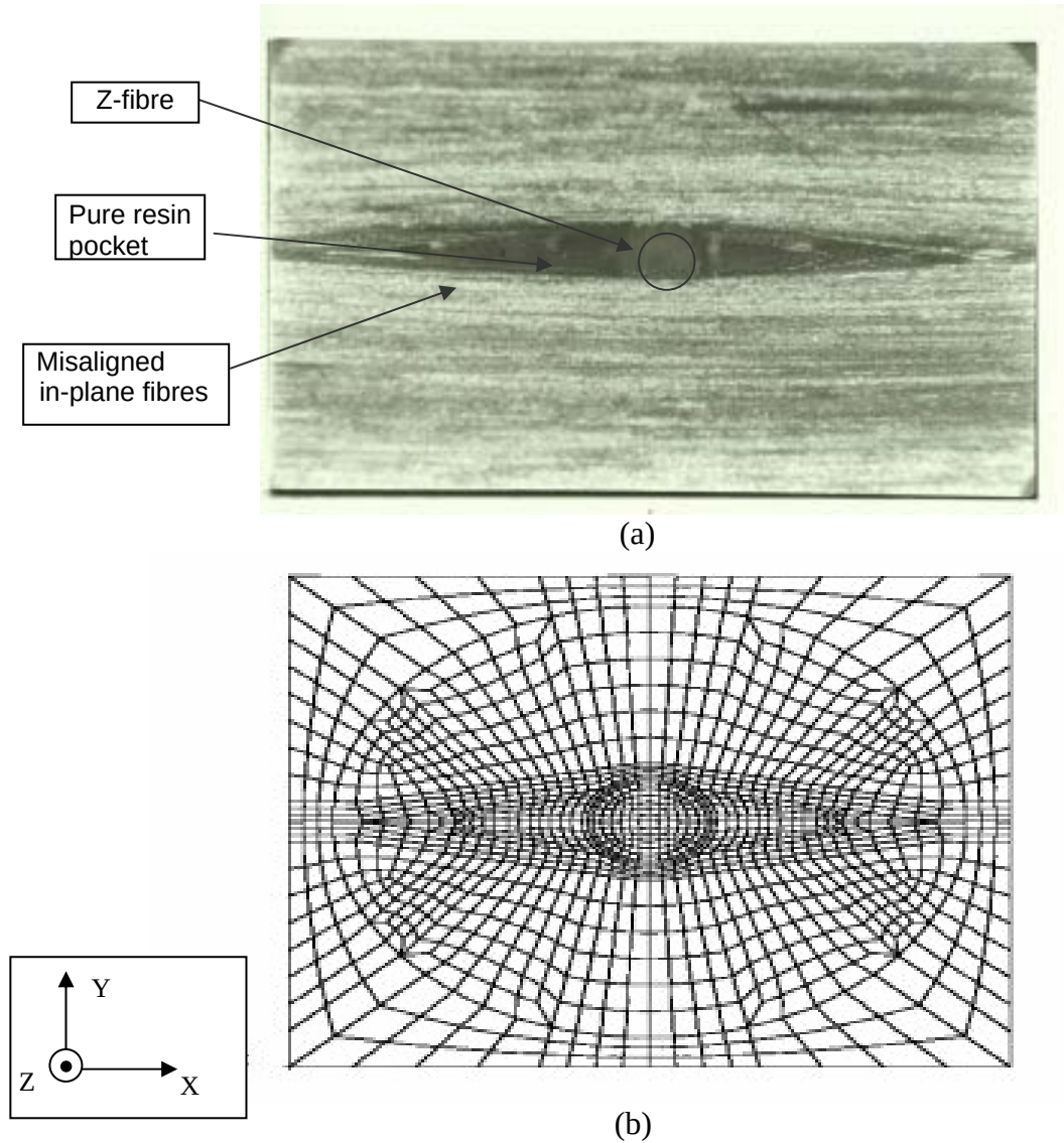
Fig. 1 (a) Microscopic photograph of a unidirectional laminate with a single z-fibre inserted; (b) 3D finite element unit cell model (XY view) used in this study.
