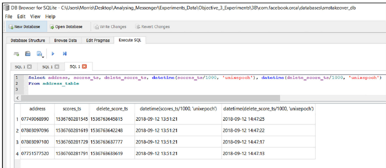
FIGURE 9 The delete_score_ts and scores_ts are stored in UNIX epoch format
