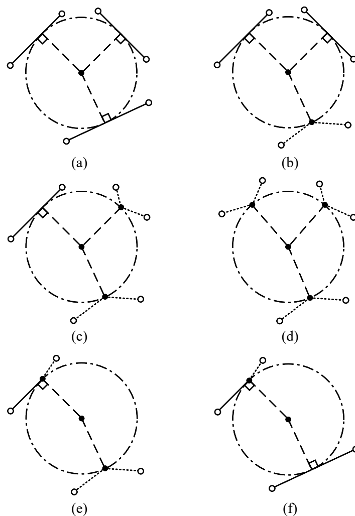
Figure 2. Illustration of maximal inscribed circle types. Two types of constraints: the circle being tangent to a segment or passing by a point. In (a), the circle is constrained by 3 segments. In (b), the circle is constrained by 2 segments and 1 extreme point. In (c), the circle is constrained by 1 segment and 2 extreme points. In (d), the circle is constrained by 3 extreme points. In (e) the circle is constrained by 1 segment and 2 extreme points, with one of the two points lying on the segment. In (f), the circle is constrained by 2 segments and 1 extreme point, which lies on one of the two segments.
