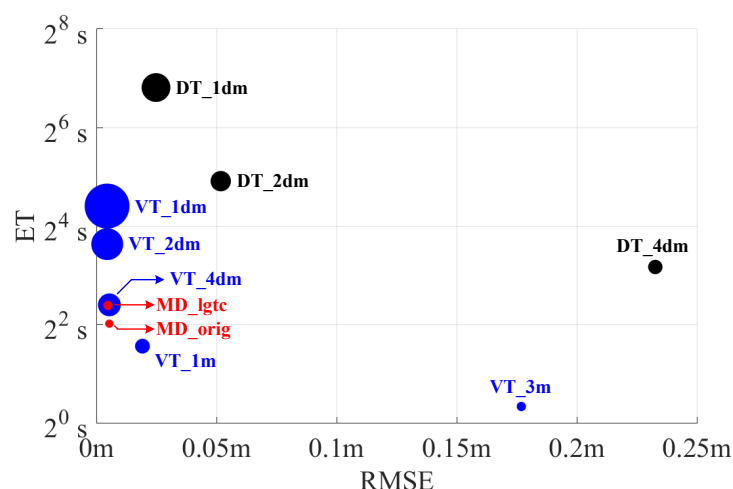
Figure 11. Illustration of performance of three methods. The ETs are plotted in binary logarithmic scale because of the huge differences in their values while various sampling resolutions are used. The radii of the circles indicate the center point numbers. The larger the radius, the more center points are.
