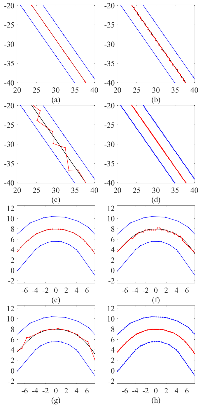
Figure 12. Illustration of the centerline extraction results of one lane. Lane boundaries are marked in blue while the ground truth and estimated centerlines are marked in black and red respectively. (a–d) show the results in the straight section and are obtained by MD_orig, DT (0.4 m), VT (original points) and VT (0.4 m) separately. (e–h) show the results in the corner section and are obtained by MD_orig, DT (0.4 m), VT (original points) and VT (1 m) separately.
