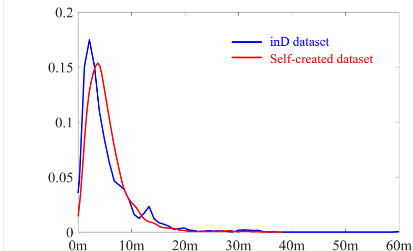
Figure 10. Illustration of KDE results of boundary segment length. The blue curve represents the inD dataset while the red one represents the self-created dataset.
