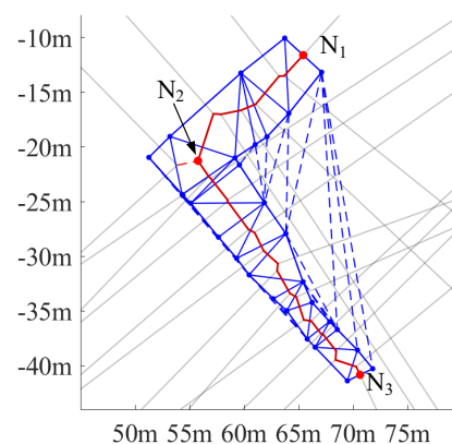
Figure 6. An illustration of the centerline (solid red segments) estimated by the VT. The grey lines are Voronoi edges perpendicular to border segments. The solid blue segments are the resulting edges from inside-lane Delaunay triangulation, while dashed blue segments are edges of Delaunay triangles outside the lane polygon. N_1 and N_3 are the start and end nodes of the centerline separately, and N_2 is a branch node. The branch node has three connected edges, one of which is a residual spur (the red dashed line).
