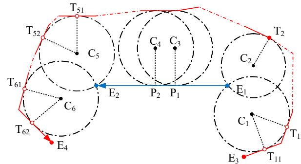
Figure 5. The left lane border, in blue, and the right lane border, in red, are oriented according to the direction of the arrows. The associated MDs are shown together with their contact points.
