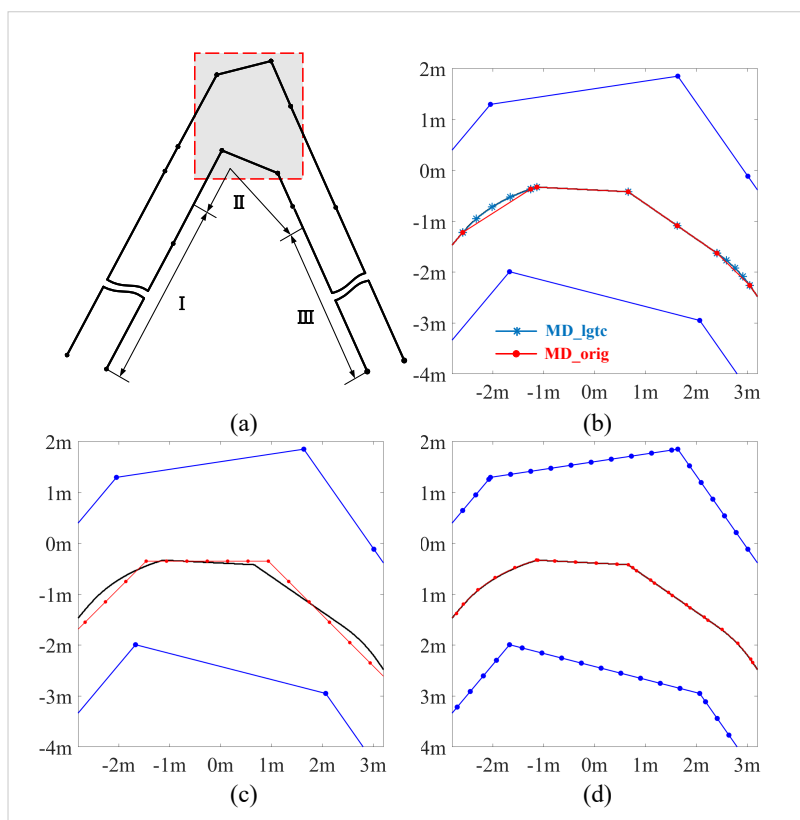
Figure 13. Illustration of centerline extraction performance in the sharp corner. (a) is the target lane and its centerline benchmark. (b–d) are results from MD, DT (0.4 m) and VT (0.4 m) separately.
