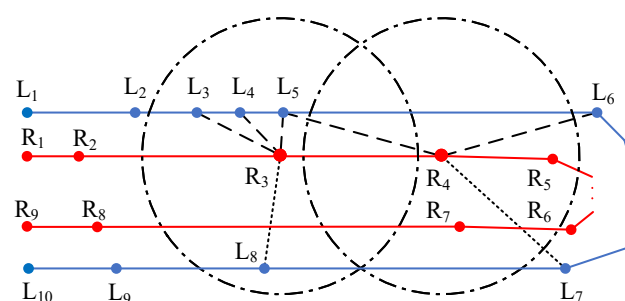
Figure 3. An illustration of a range search and a nearest-neighbor search, based on point R_3 and point R_4 separately. Blue line segments belong to the left lane border while red ones belong to the right lane border. In the range search, R_3 should be matched with L_3 , L_4 and L_5 , but not L_8 . In the nearest neighbor search, R_4 should be matched with L_5 , and L_6 , but not L_7 .
