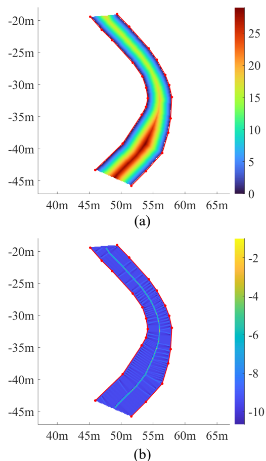
Figure 7. Visualization of the results of the intermediate steps of centerline extraction based on DT. (a) The distance map. (b) The ridge map.
