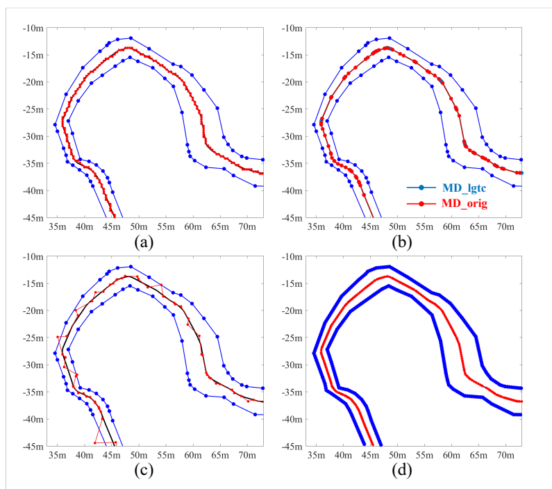
Figure 15. Illustration of centerline extraction performance in the lane with varying widths. (a–d) are results from DT (0.4 m), MD, VT (original points) and VT (0.4 m) separately. The lane boundaries are marked in blue and the ground truth centreline is in black, while the estimated centerline is in red.
