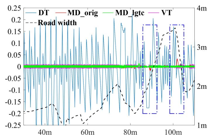
Figure 16. The deviation from the calculated centerline to the benchmark centerline. The green, red, pink and blue lines are from MD_lgtc, MD_orig, VT and DT separately. The black dashed line is the road width along the lane
