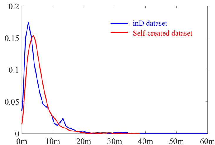
Figure 10. Illustration of KDE results of boundary segment length. The blue curve represents the inD dataset while the red one represents the self-created dataset.
