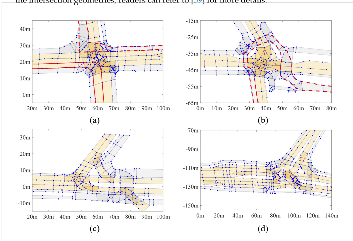
Figure 9. The four scenarios in the inD are illustrated in (a–d). Sparse points are marked in blue. Lanelets are represented by polygons. Vehicle driving lanes and non-driving lanes (like pedestrian paths) are marked in light yellow and grey separately. Examples of a complete pedestrian path and a driving lane are bounded by solid and dashed red lines separately.
