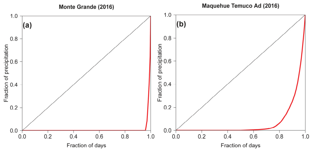
Figure 4. Lorenz curve for two pluviographic stations for the year 2016, in the study area. (a) Monte Grande pluviographic station; (b) Maquehue Temuco Ad pluviographic station.
