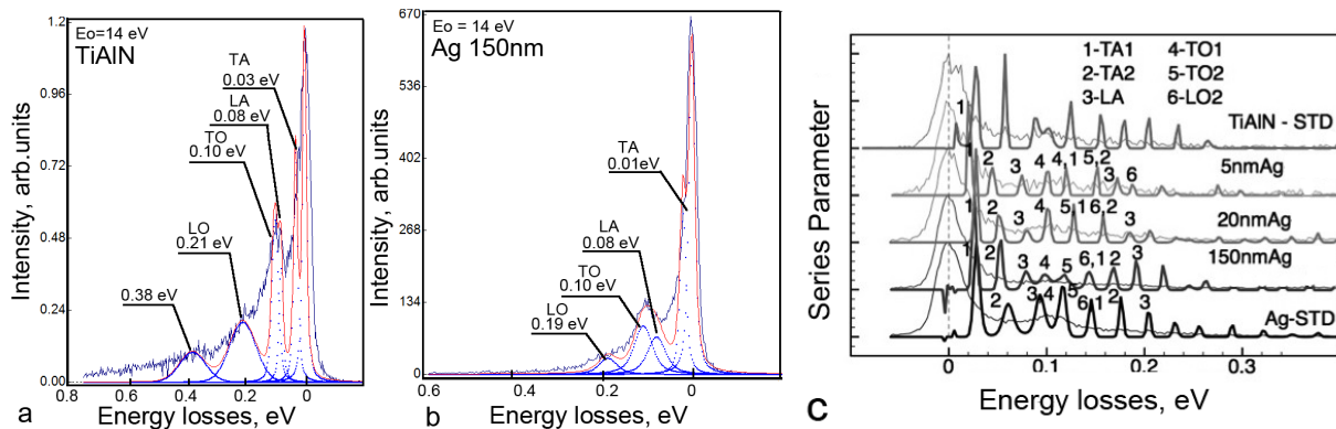
Figure 2. Experimental phonon spectra from TiAlN layer (a) and 150nm Ag layer (b) in multilayer coating; c - deconvolution of REELS for investigated specimens. Note that the scattering geometry employed in the present work corresponds to maximal intensity of phonon excitation ( E_0 = 14 \text{ eV} ).
