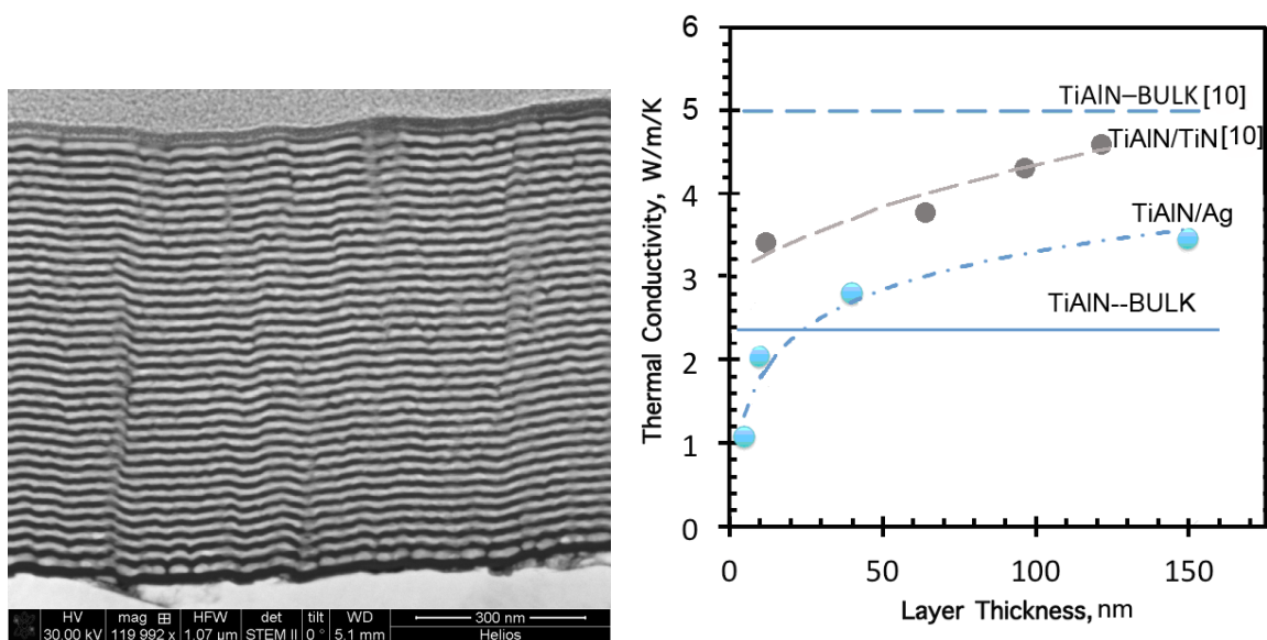
Figure 1. a – STEM cross-sectional image showing the structure of a TiAlN/Ag multilayer coating with 35 bilayers prepared by DC magnetron sputtering; b – The influence of the Ag film thickness on the thermal conductivity coefficient of TiAlN/Ag. These data are compared with literature ones for TiAlN/TiN coatings [10]
