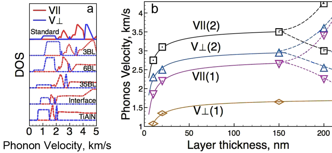
Figure 3. (a) Density of the states (DOS) of acoustic phonons and (b) dependence of Ag (TA) phonons velocity with Ag layer thickness in TiAlN/Ag coatings.
