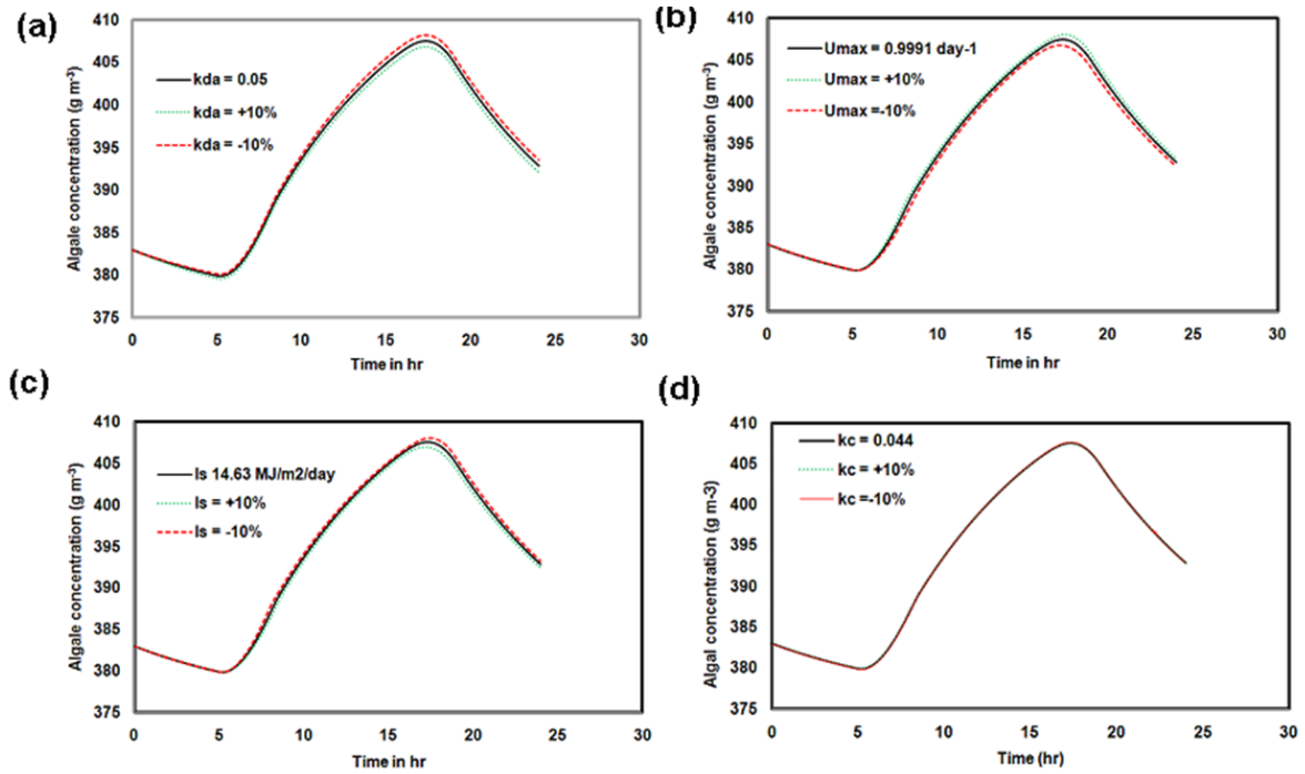
Figure 7: Sensitivity analysis of (a) decay rate (b) maximum specific growth rate (c) saturation light intensity (d) nutrient half saturation constant on algal biomass concentration
