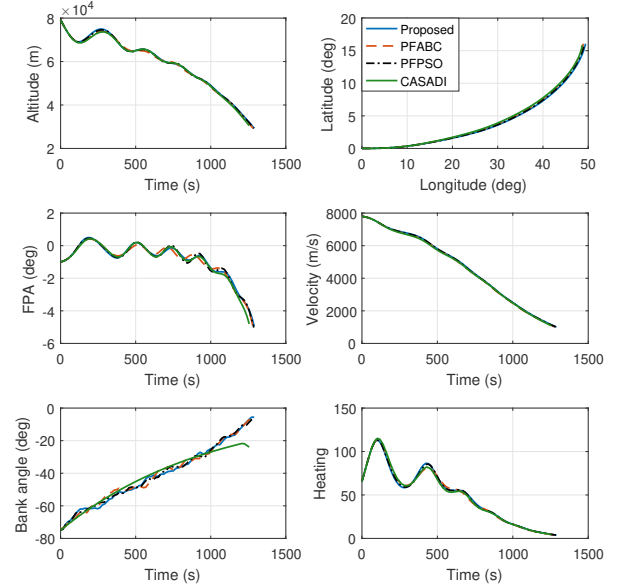
Fig. 4: State/control/constraint evolutions: Case 3
