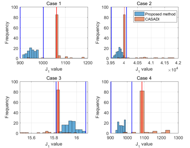
Fig. 6: Histograms of J_1 for the two methods
