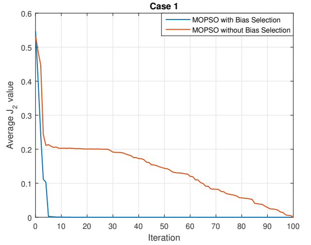
Fig. 10: Experiment 1: J_2 results for mission case 1
