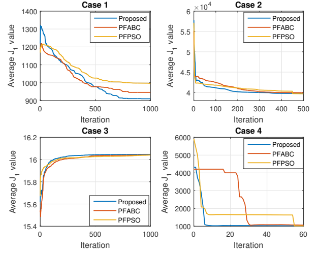
Fig. 9: J_1 evolutions: Cases 1-4
