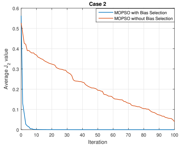
Fig. 11: Experiment 1: J_2 results for mission case 2
