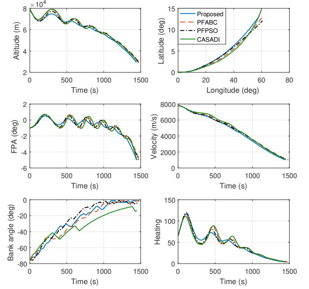
Fig. 3: State/control/constraint evolutions: Case 2
