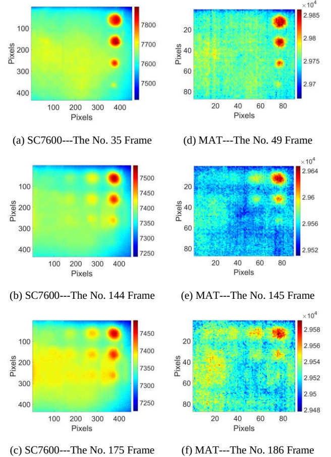
Fig. 4. The raw thermal images at different times for Sample 1.
