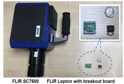
Fig. 2. Comparison of the FLIR lepton with SC7600 for active thermography
