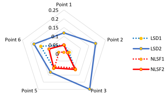
Fig. 6 The error range of FLIR SC7600 and MAT system using LSD and NLSF methods, where LSD1 and NLSF1 come from FLIR SC7600 (dash line), and LSD2 and NLSF2 come from MAT(solid line).
