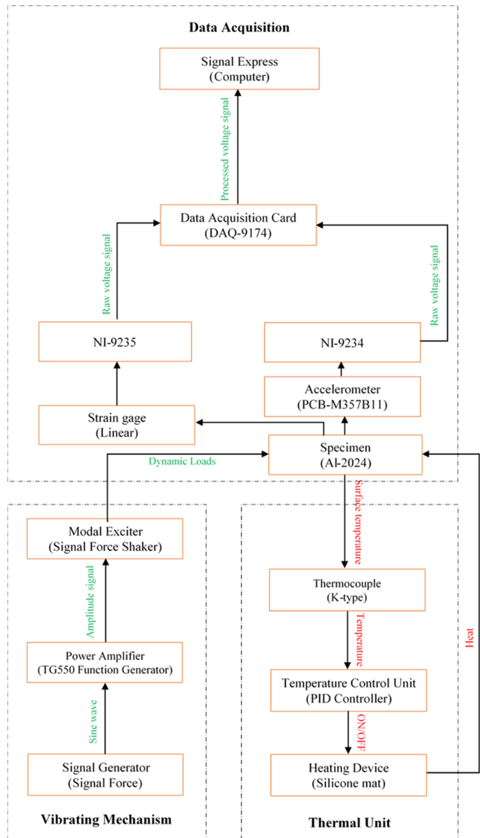
Figure 4. Experimental layout.
