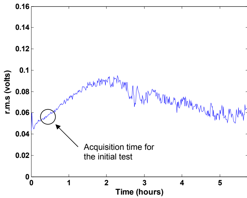
Figure 19 Continuous AE r.m.s values for no-load condition.
