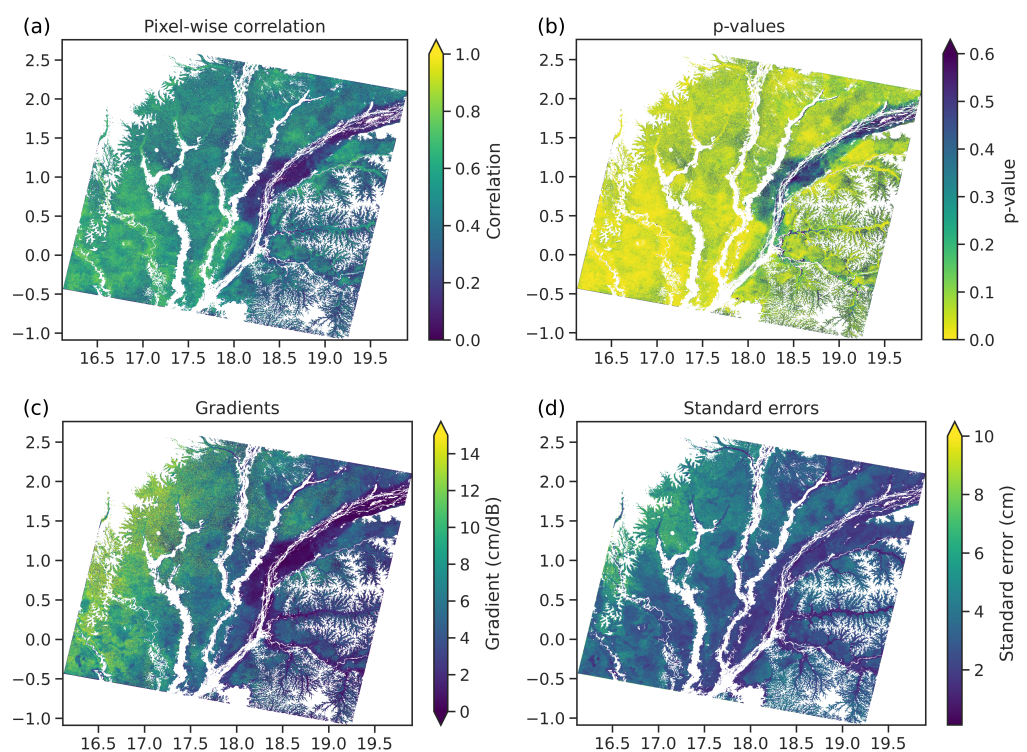
Figure 6. Pixel-wise correlations calculated between time series of the change in SAR backscatter between subsequent PALSAR-2 scenes, \delta HH , and the corresponding net water accumulations across the ALOS-2 PALSAR-2 HH backscatter stack. (a) Correlations, (b) p -values, (c) gradients and (d) standard errors of the pixel-wise correlation. Permanent water bodies and non-peatland land cover have been masked.
