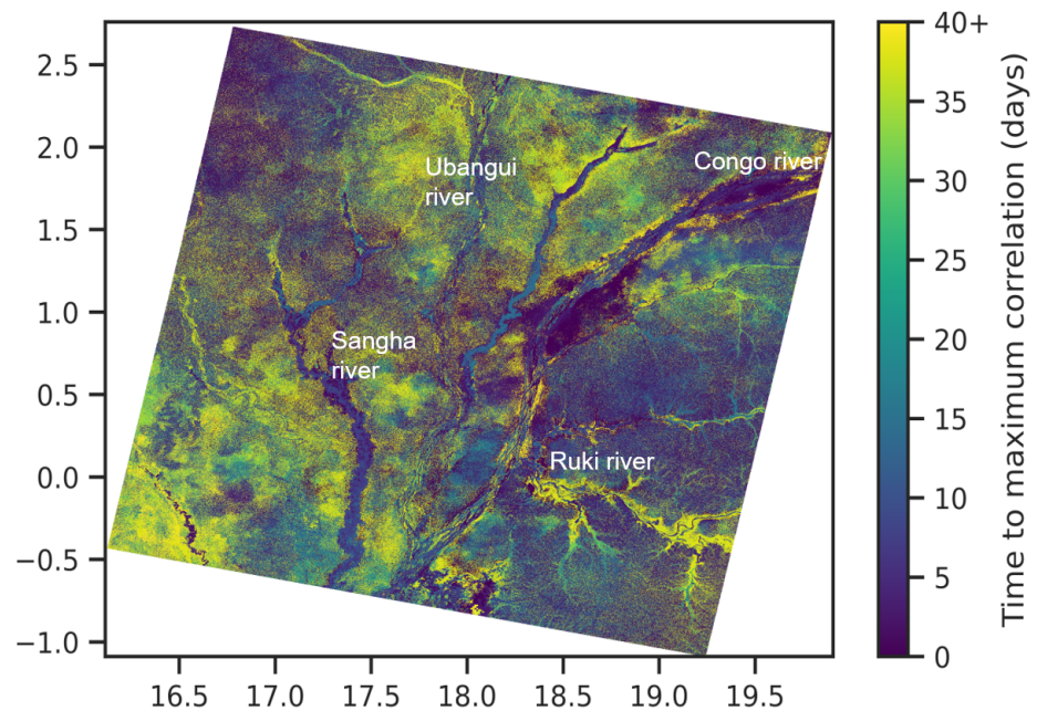
Figure 8. The period of maximum correlation across the extent of the study area—the number of days of net water accumulation that result in the maximum correlation between the ALOS-2 PALSAR-2 HH backscatter and the net water time-series data.
