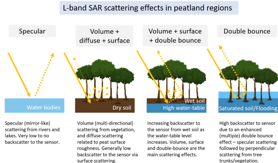
Figure 2. Summary of the backscattering mechanisms involved between L-band SAR data and regions of tropical peatland.
