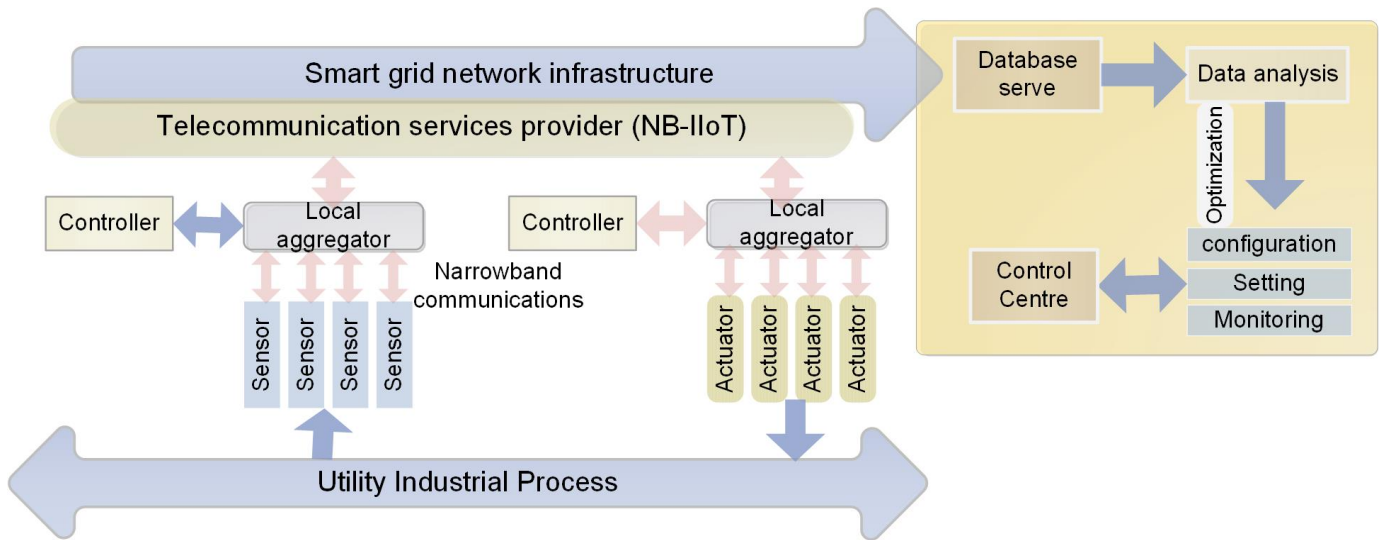
Fig. 4. Industrial process system.
