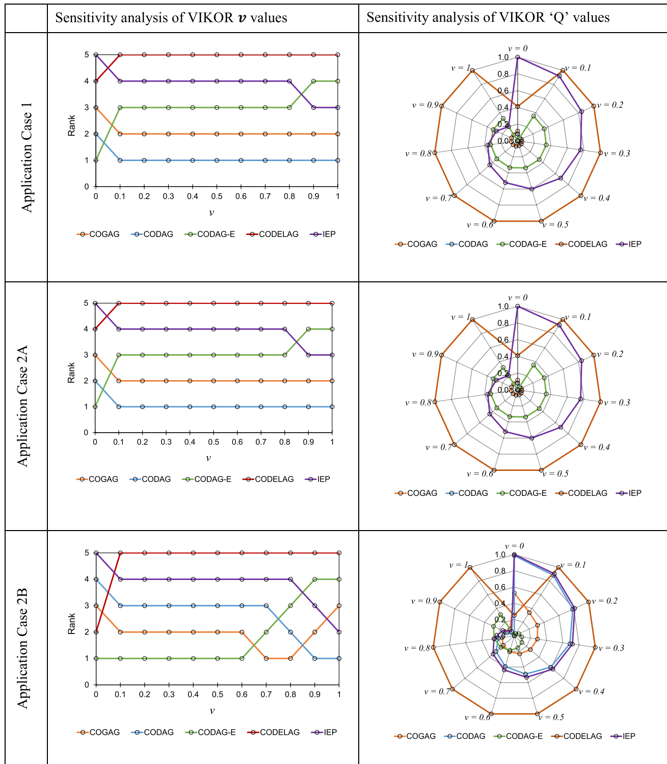
Fig. 30 Sensitivity analysis of VIKOR v, Q values for the Application Cases
