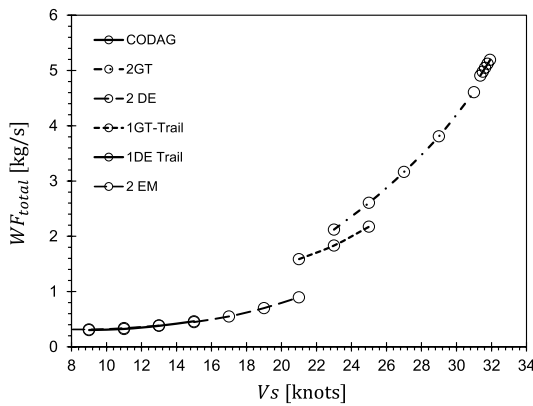
Candidate architecture: A3 CODAG-E
