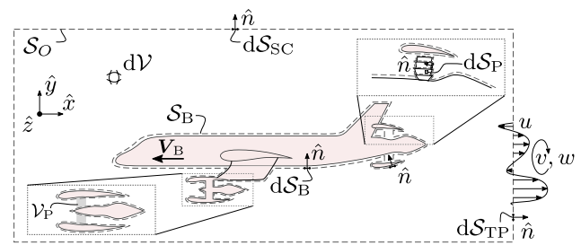
Fig. 2 Schematic of a control volume encapsulating a powered aerodynamic body
