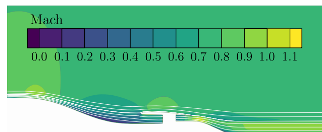
Fig. 11 Mach number contours around a propulsive fuselage concept, with streamlines through the propulsor and over its cowl
