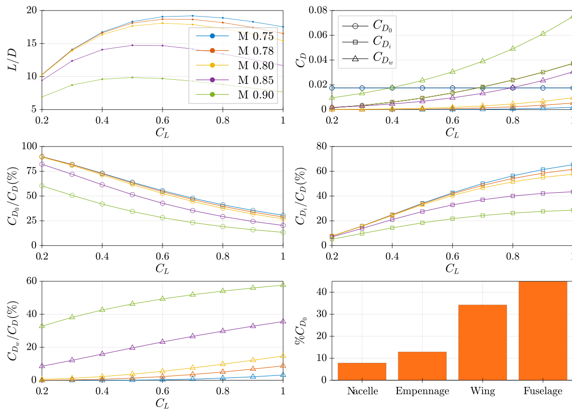
Fig. 17 Drag build-up of the reference aircraft, for an assumed lift-to-drag ratio L/D = 19.0 at M_B 0.78 , corresponding to a lift coefficient of C_L = 0.6
