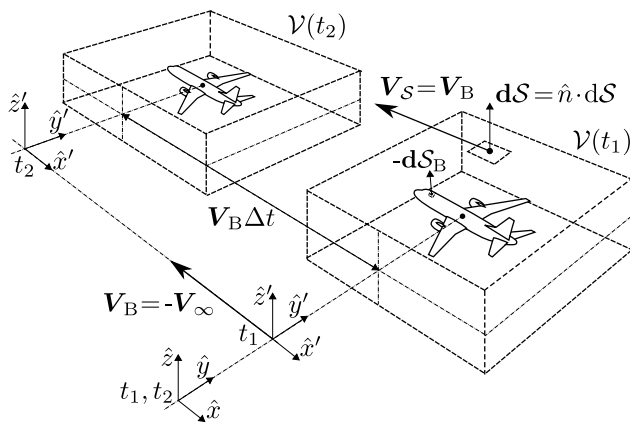
Fig. 1 Motion of a flying aircraft from t_1 to t_2 with its control volume in the ARF ( \hat{x}, \hat{y}, \hat{z} ) and the RRF ( \hat{x}', \hat{y}', \hat{z}' , from Ref. [16]). Source: Adapted with permission from Sanders, D. S., “Aircraft Aerodynamic Work-Energy Relationships with Mass Source Considerations,” Tech. Rep. RP0028, Cranfield University, Cranfield, United Kingdom, 2023
