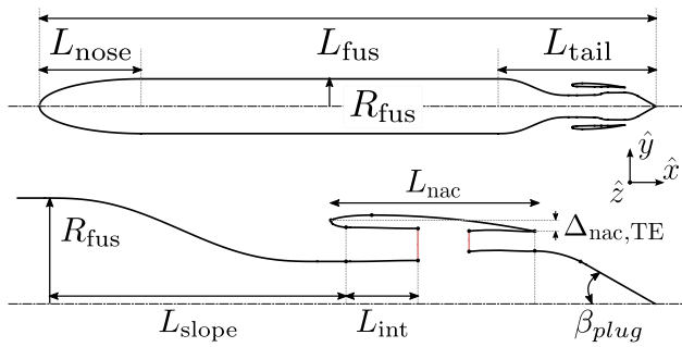
Fig. 6 Schematic of an axi-symmetric propulsive fuselage concept and its parametrisation
