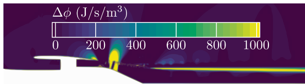
Fig. 14 Difference in local volume-specific viscous dissipation rate for fan polytropic efficiencies of 90% and 95% on the baseline thruster
