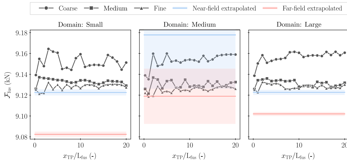
Fig. 16 Comparison of net stream-wise force between the near-field and far-field , as computed, and their extrapolated values from the Table 1
