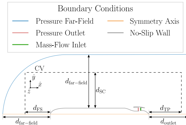
Fig. 8 Schematic of the domain, propulsive fuselage model, boundary conditions and analysis control volume
