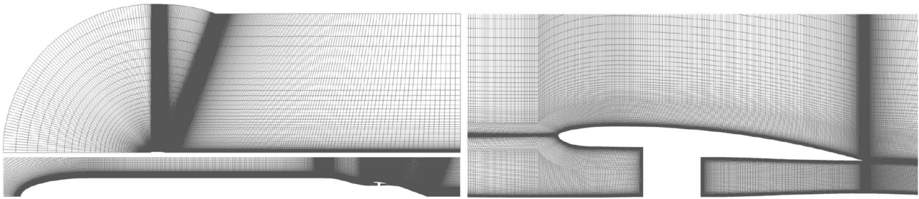
Fig. 7 C-grid around a propulsive fuselage with the domain's mesh, around the fuselage and the propulsor
