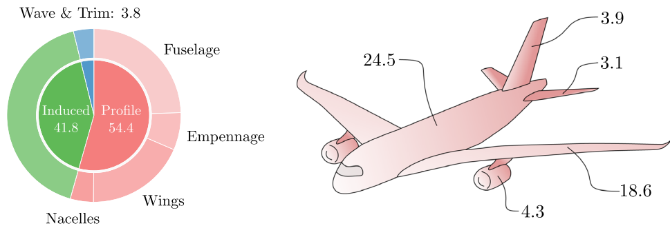
Fig. 10 Aircraft profile, lift-induced and wave drag shares (left), and aircraft components' portions of profile drag (right)
