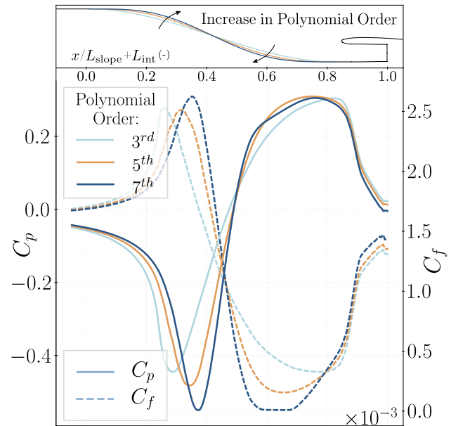
Fig. 15 Local pressure and skin-friction coefficients distribution along the pre-diffusive slope for different curve polynomial orders
