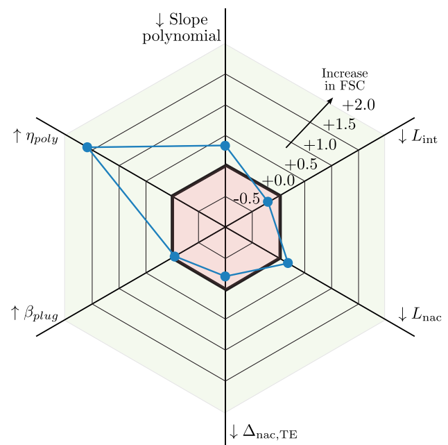
Fig. 13 Sensitivity of the fuel saving coefficient, with gain in green and loss in red, to changes in thruster design variables (rises \uparrow , or decreases \downarrow ) from the baseline configuration with FSC = 10.5%
