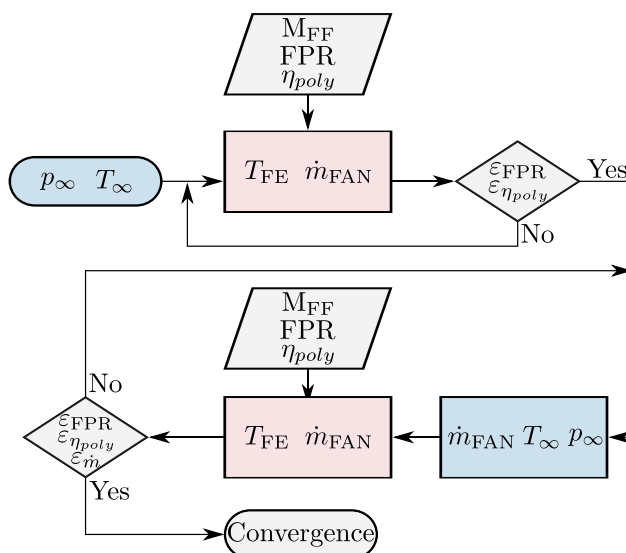
Fig. 9 Fan modelling iterative procedure within the CFD with conditions at the fan-face (blue) and fan-exit (red)
