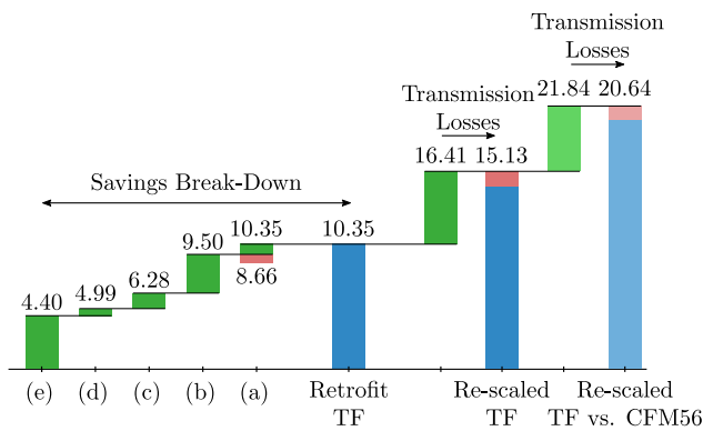
Fig. 12 Power saving coefficient sensitivity to different propulsion system efficiencies
