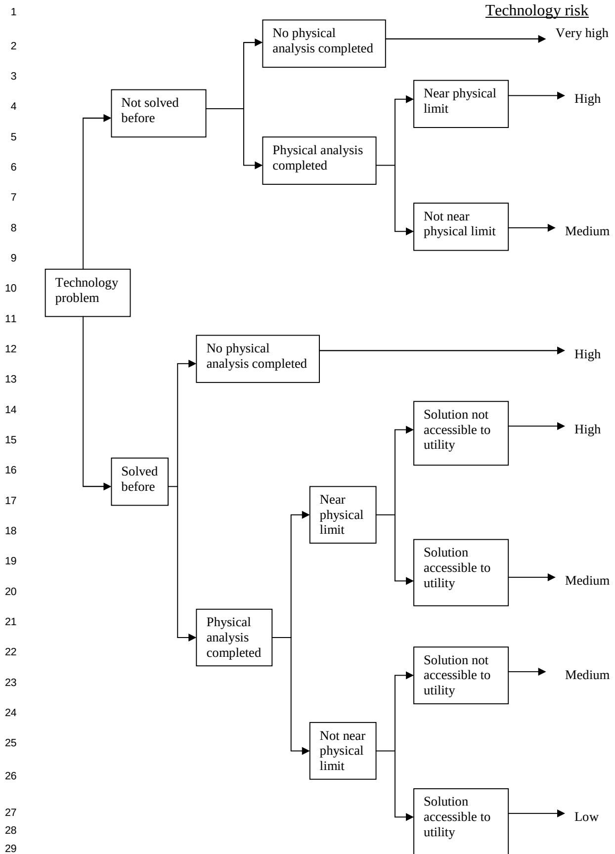
Figure 3. Technology risk algorithm (Hartmann and Lakatos 62 with permission).
