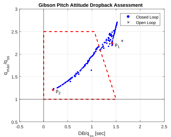
Fig. 8. Gibson Pitch Attitude Drop-back Assessment
