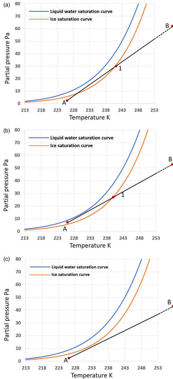
Figure 5. No contrail formation.
