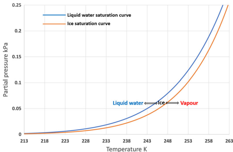
Figure 2. Water phase diagram (below 273.15K).
