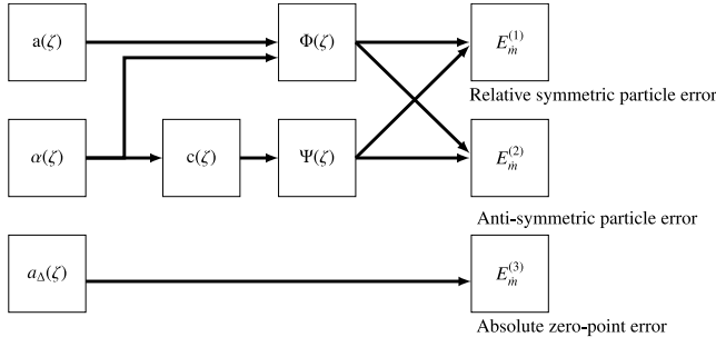
Fig. 3. Influence diagram of external factors on the mass flow error contributions. The axial dependence of the particle radius a and the particle fraction \alpha lead to the force perturbations \Psi and \Phi , which in turn cause the measurement errors E_m^{(1)} and E_m^{(2)} . The asymmetry of the moment of inertia, a_\Delta leads to an additional measurement error E_m^{(3)} .
