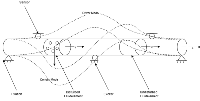
Fig. 2. Schematic description of the first symmetric (driver) and anti-symmetric (Coriolis) mode of the measurement tube: shown are the relevant mechanical components as sensors and exciters as well as the two different kind of fluid elements: homogeneous (single-phase) and mixed (with entrained particles) with a fluid speed v .
