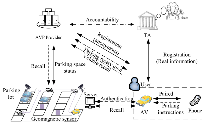
FIGURE 3. AVP architecture.
