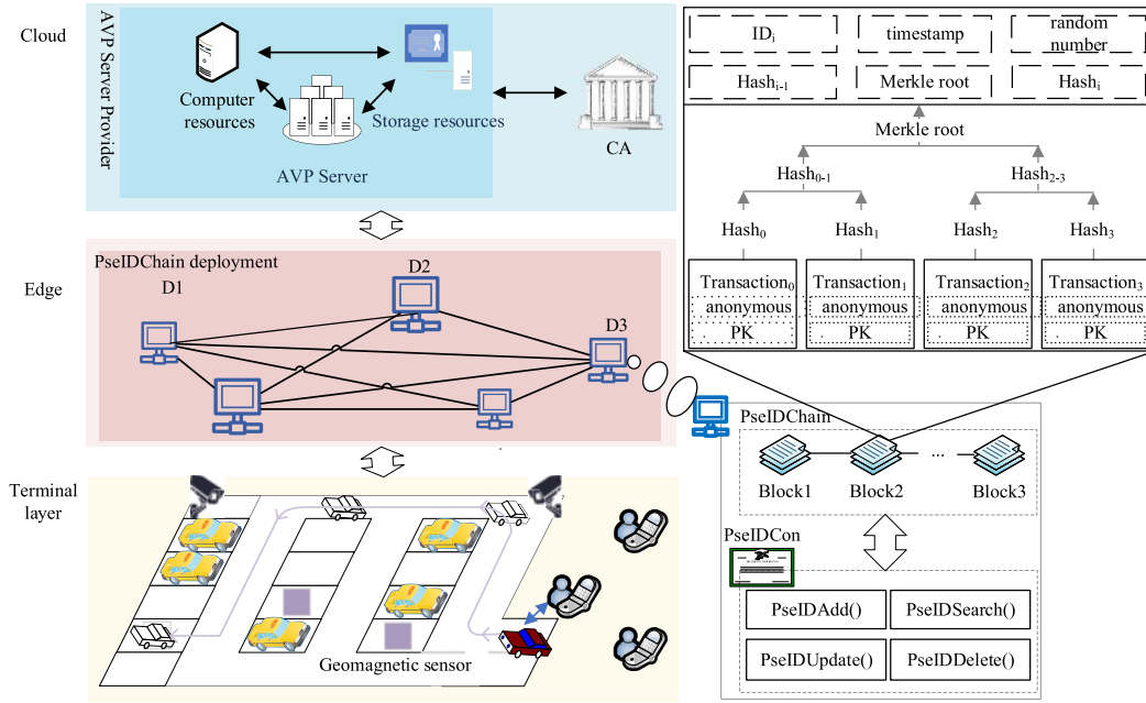
FIGURE 4. System model.
