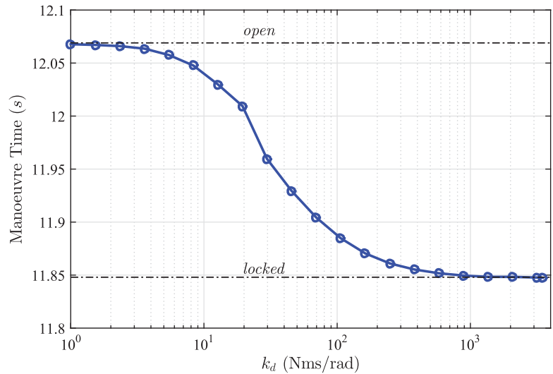
Figure 4. Manoeuvre time sensitivity analysis (speed sensing configuration).
