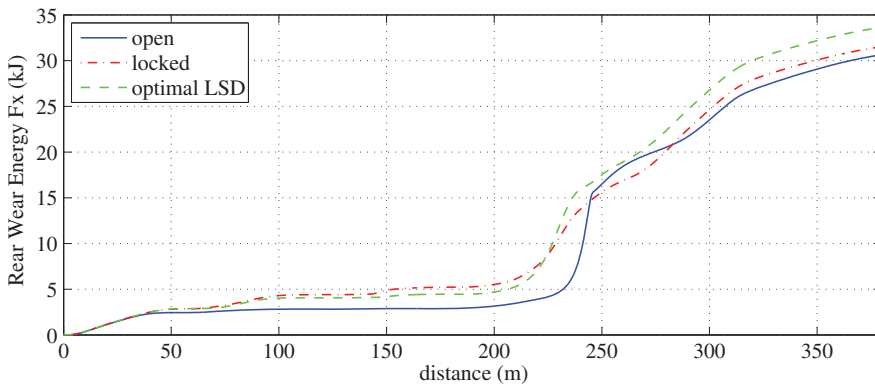
Figure 9. Total driven wheel tyre wear energy, W_{f_{\text{rear}}} .
