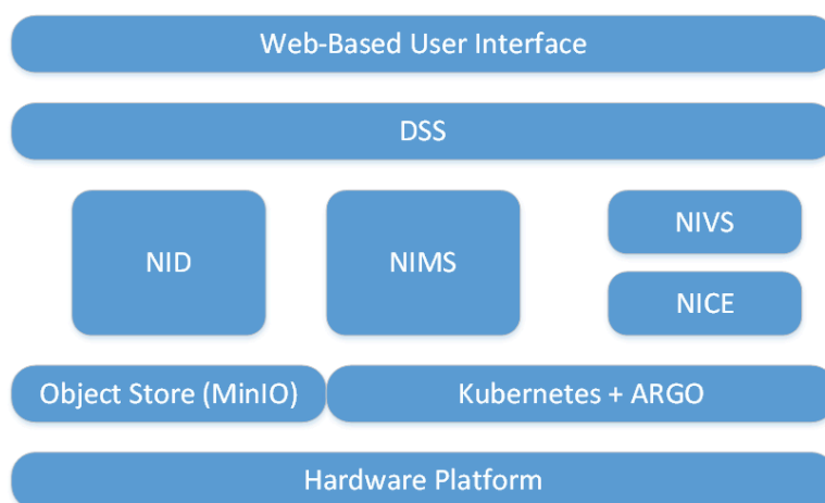
Figure 1. Dafni core components
