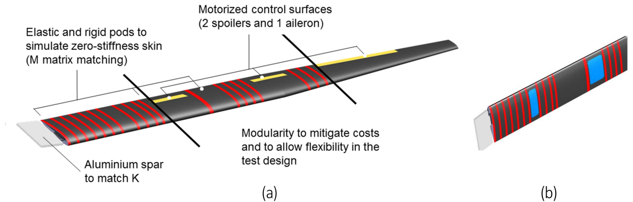
Figure 19. XB-2 Preliminary Design for Manufacture
