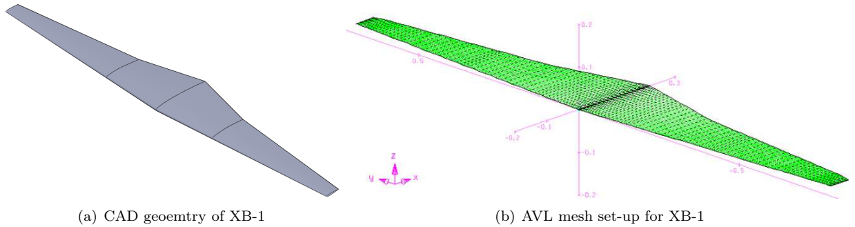
Figure 7. Athena Vortex Lattice (AVL) code set up for XB-1 analysis
