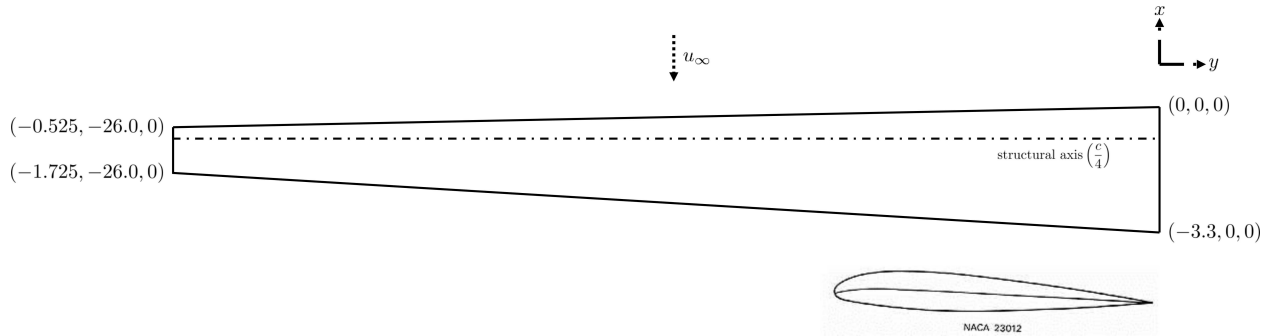
Figure 17. XB-2 Planform Definition
